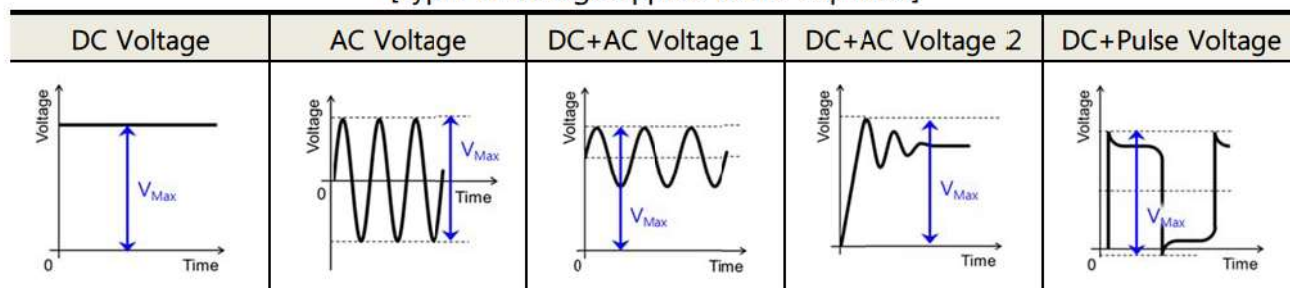
[Types of Voltage Applied to the Capacitor]
