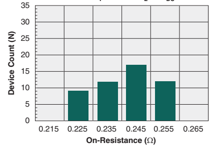
Typical On-Resistance Distribution (N=50, I F =10mA, I L =1A DC )
