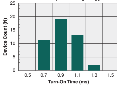
Typical Turn-On Time (N=50, I F =10mA, I L =1A DC )
