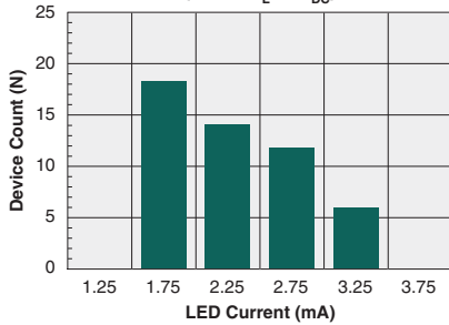
Typical I F for Switch Operation (N=50, I L =1A DC )
