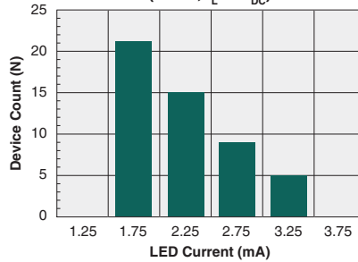
Typical I F for Switch Dropout (N=50, I L =1A DC )
