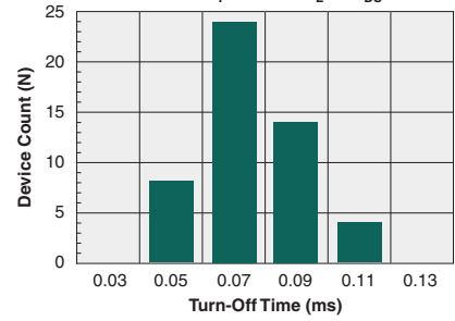
Typical Turn-Off Time (N=50, I F =10mA, I L =1A DC )
