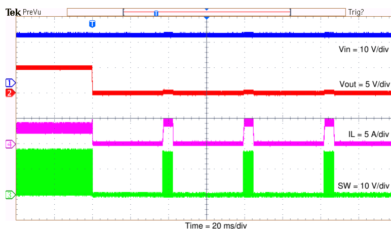
Figure 5-14. TPS56339EVM Short Protection
