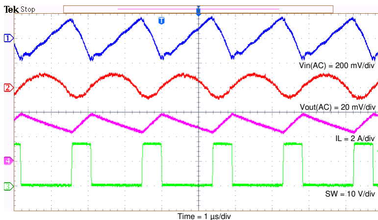
Figure 5-7. TPS56339EVM Output Ripple, I_{OUT} = 3 A
