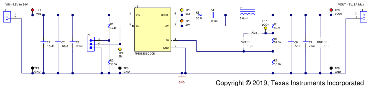
Figure 7-1. TPS56339EVM Schematic
