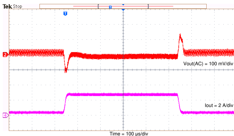
Figure 5-6. TPS56339EVM Transient Response 0.3 to 2.7 A
