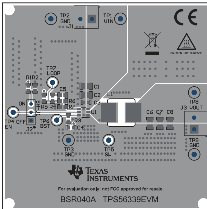
Figure 6-1. Top Assembly
