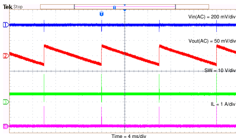
Figure 5-9. TPS56339EVM Output Ripple, I_{OUT} = 0 A
