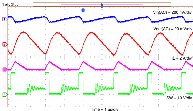
Figure 5-8. TPS56339EVM Output Ripple, I_{OUT} = 0.3 A
