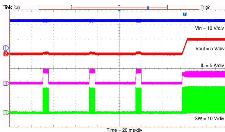
Figure 5-15. TPS56339EVM Short Recovery
