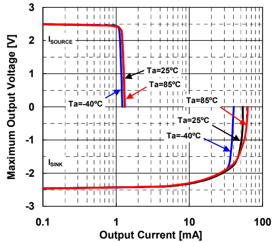
Maximum Output Voltage vs. Output Current (Temperature) V^*/V = \pm 2.5V , G_v = \text{open}
