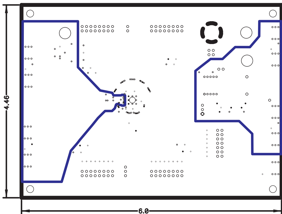
Figure A-5. Power Plane 1
