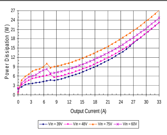
Power Dissipation vs. Vin (test in socket, no base-plate)
