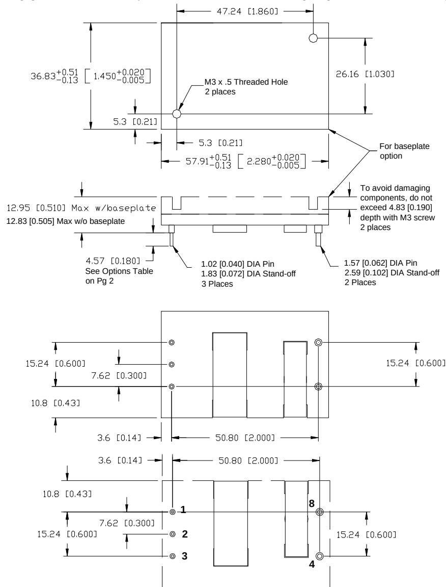
Recommended hole pattern (top view)
