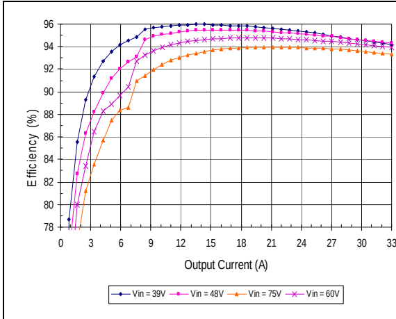
Typical Efficiency vs. Vin (test in socket, no base-plate, Vo measured at socket terminals)
