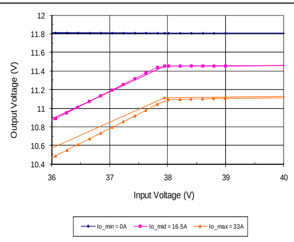
Output Voltage vs. Vin (between 36V and 40V)
