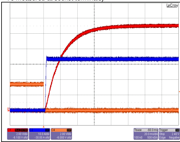
Start-up from on/off Switch at Vin,nom and Full Load. Ch. 1: Vo Ch. 2: Io Ch. 4: ON/OFF
