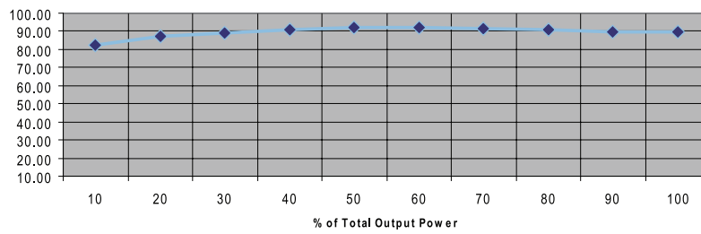
230 Vac Efficiency
