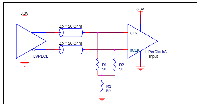
FIGURE 2B. HiPERCLOCK ® CLK/nCLK INPUT DRIVEN BY 3.3V LVPECL DRIVER
