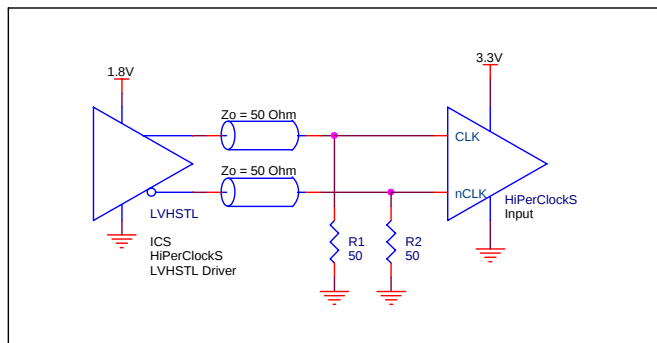
FIGURE 2A. HiPERCLOCK SM CLK/nCLK INPUT DRIVEN BY IDT HiPERCLOCK SM LVHSTL DRIVER
