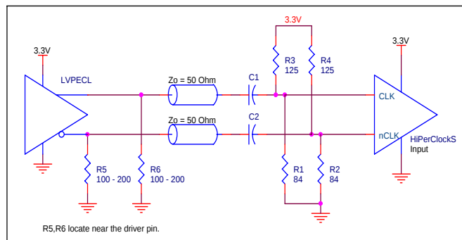
FIGURE 2E. HiPERCLOCK ® CLK/NCLK INPUT DRIVEN BY 3.3V LVPECL DRIVER WITH AC COUPLE
