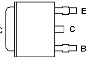
Pin Out Configuration Top View
