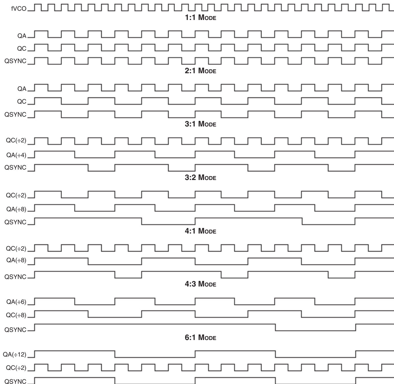
FIGURE 1. TIMING DIAGRAMS
