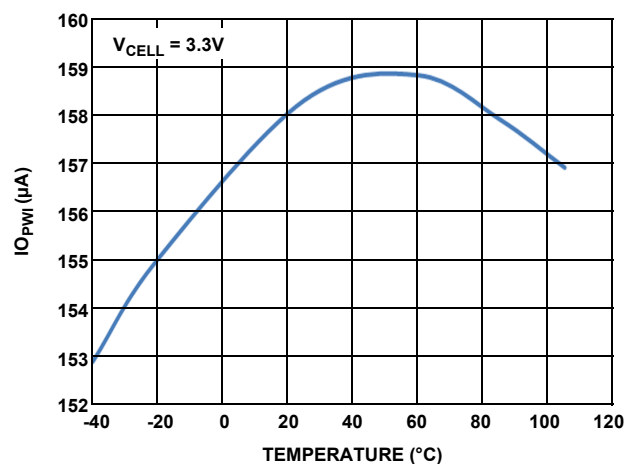
Figure 18. Open-Wire Test Current vs. Temperature (150μA Setting)
