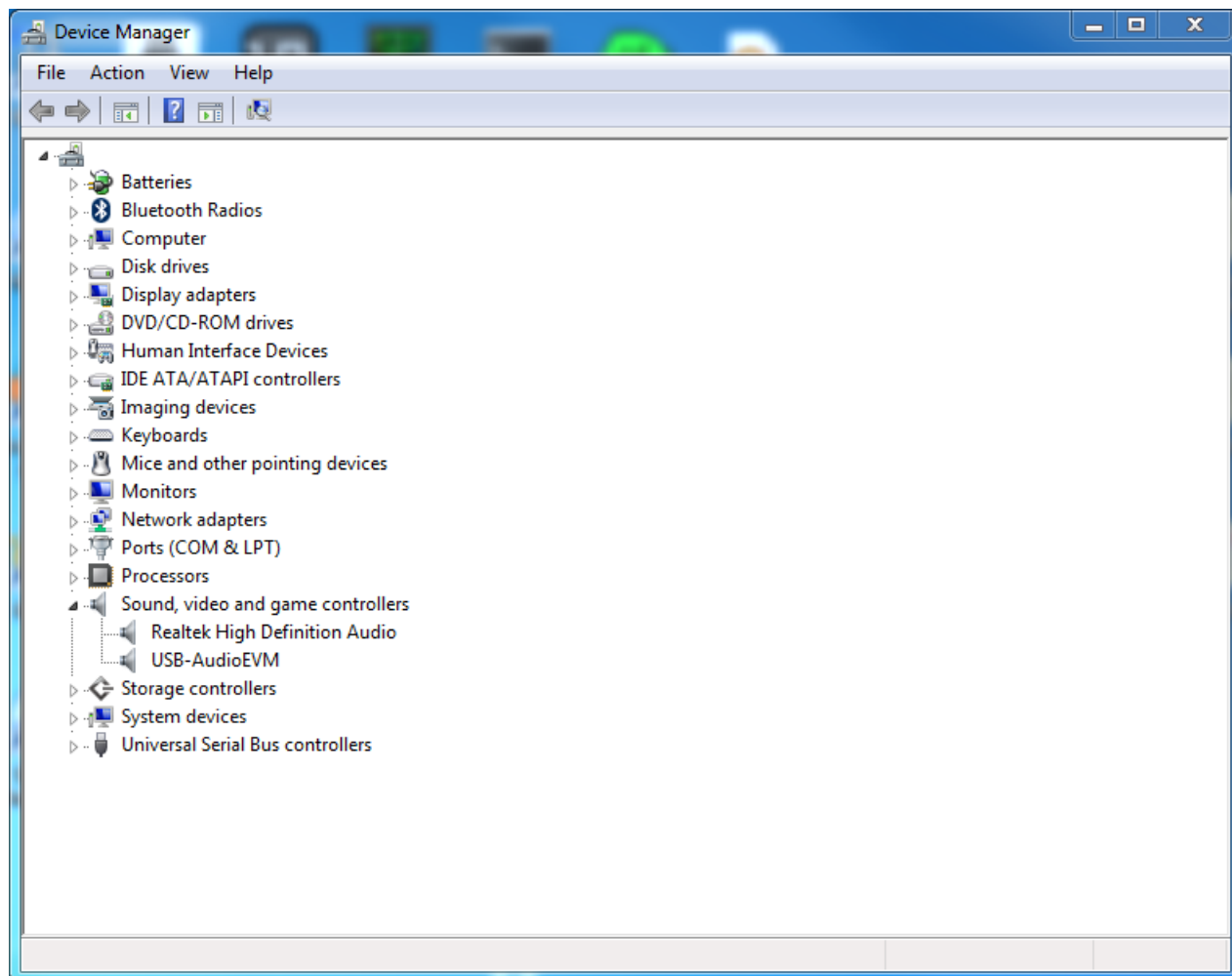
Figure 2. Device Manager
