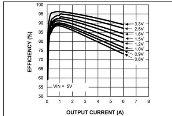
FIGURE 2-24: Efficiency ( V_{IN} = 5V ) vs. Output Current.
