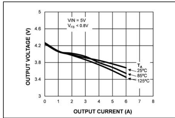
FIGURE 2-23: Output Voltage ( V_{IN} = 5V ) vs. Output Current.
