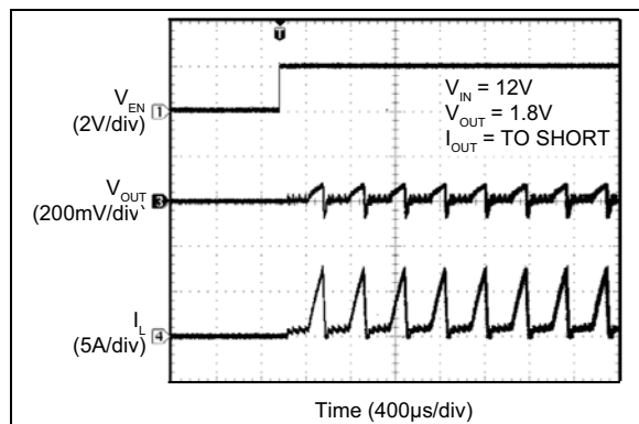
FIGURE 2-43: Enable Into Short Circuit.
