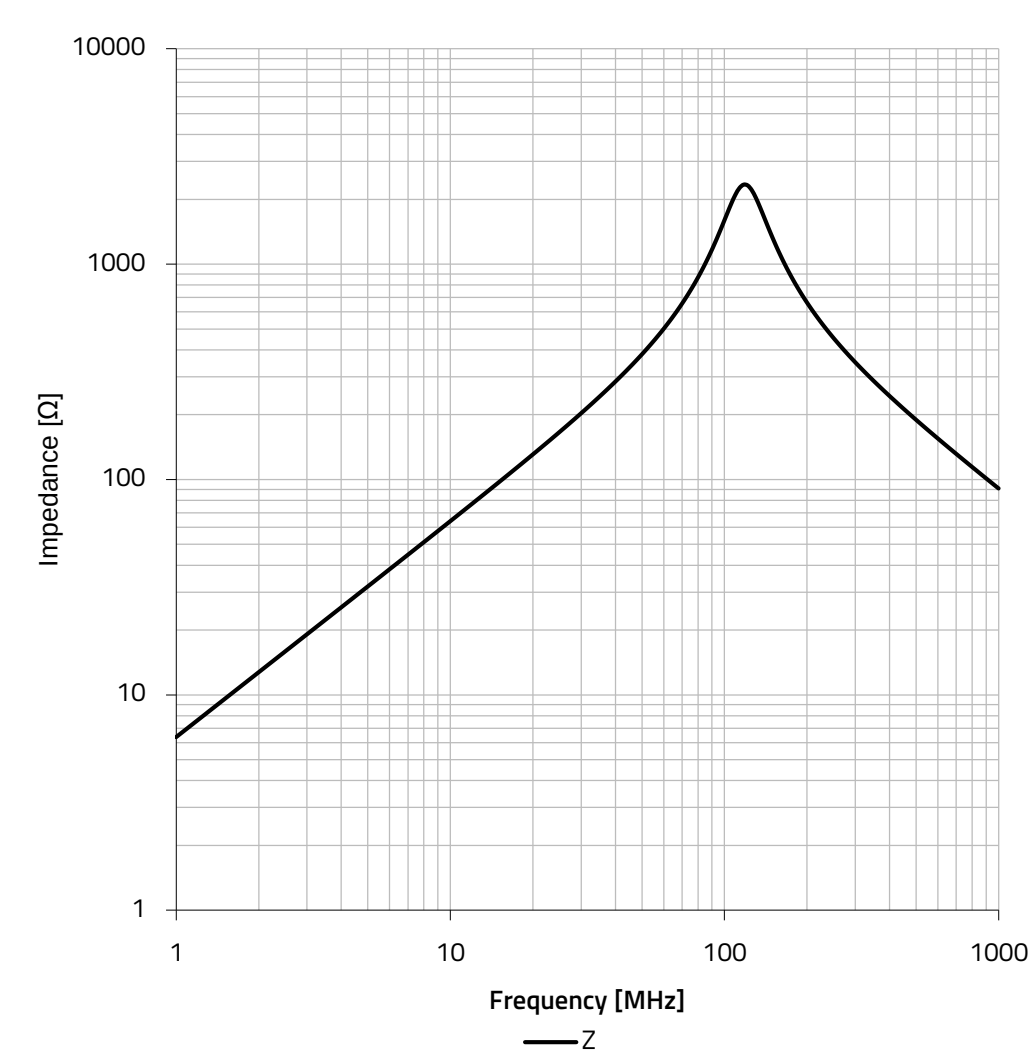
Typical Impedance Characteristics:
