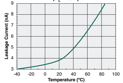
Leakage Current vs. Temperature Measured Across Pins 5&6 ( V_L=400V )
