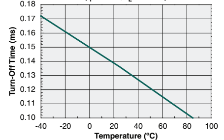
Typical Turn-Off Time vs. Temperature ( I_F=5\text{mA} , I_L=80\text{mA} )
