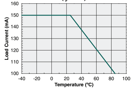
Maximum Load Current vs. Temperature AC/DC Configuration ( I_F=5mA )
