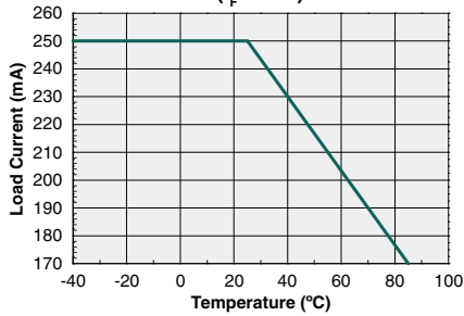
Maximum Load Current vs. Temperature DC-Only Configuration ( I_F=5mA )
