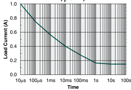
Energy Rating Curve, Single Pole ( I_F=5mA )
