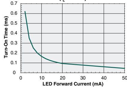
Typical Turn-On Time vs. LED Forward Current ( I_L=30\text{mA} )
