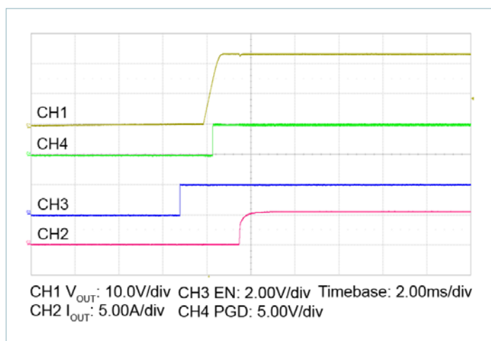
Figure 10 — Start-up with 48V IN to 24V OUT at 5.42A, Ext C SS = 0μF
