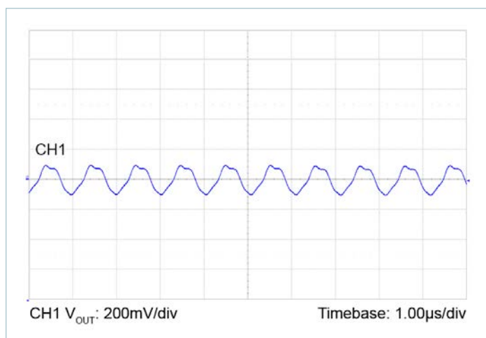
Figure 11 — Output voltage ripple at 48V IN to 24V OUT , 5.42A; C OUT = 8 x 2.2μF Ceramic
