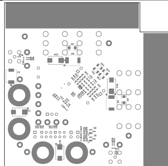
MAX20808 EV Kit PCB Layout—Bottom
