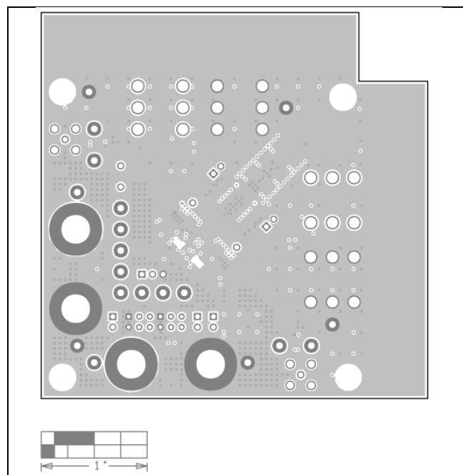
MAX20808 EV Kit PCB Layout—Layer 2
