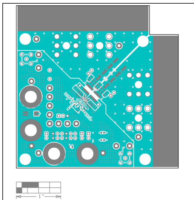
MAX20808 EV Kit PCB Layout—Top
