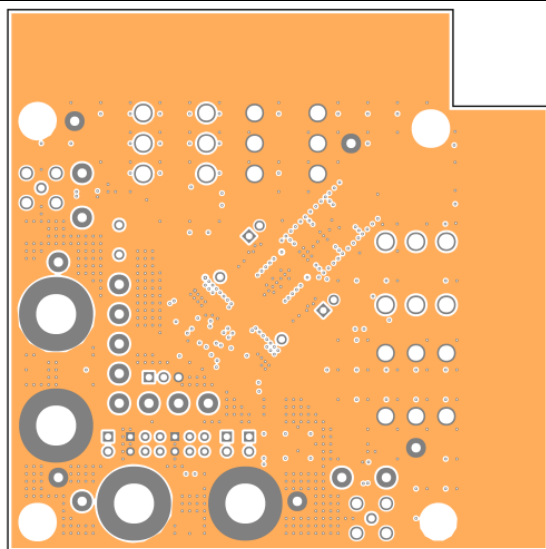
MAX20808 EV Kit PCB Layout—Layer 4
