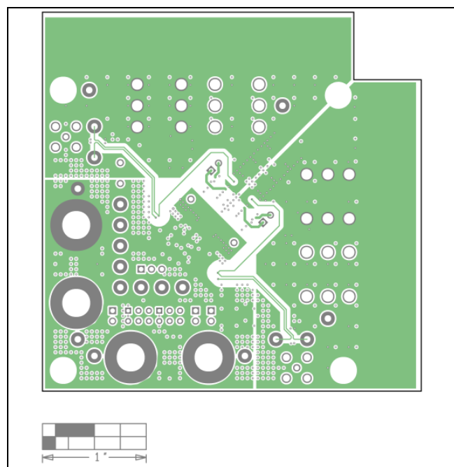
MAX20808 EV Kit PCB Layout—Layer 3
