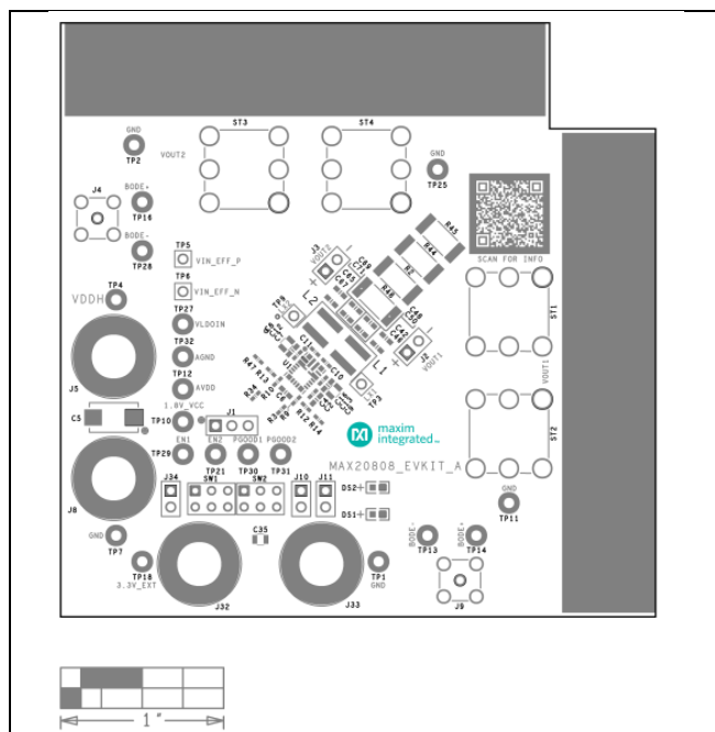
MAX20808 EV Kit Component Placement Guide—Top Silkscreen
