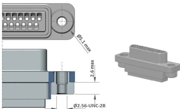
Captive Nut (Option E)
