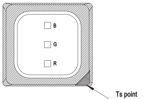
Figure 17: Solder Point Temperature on PCB
