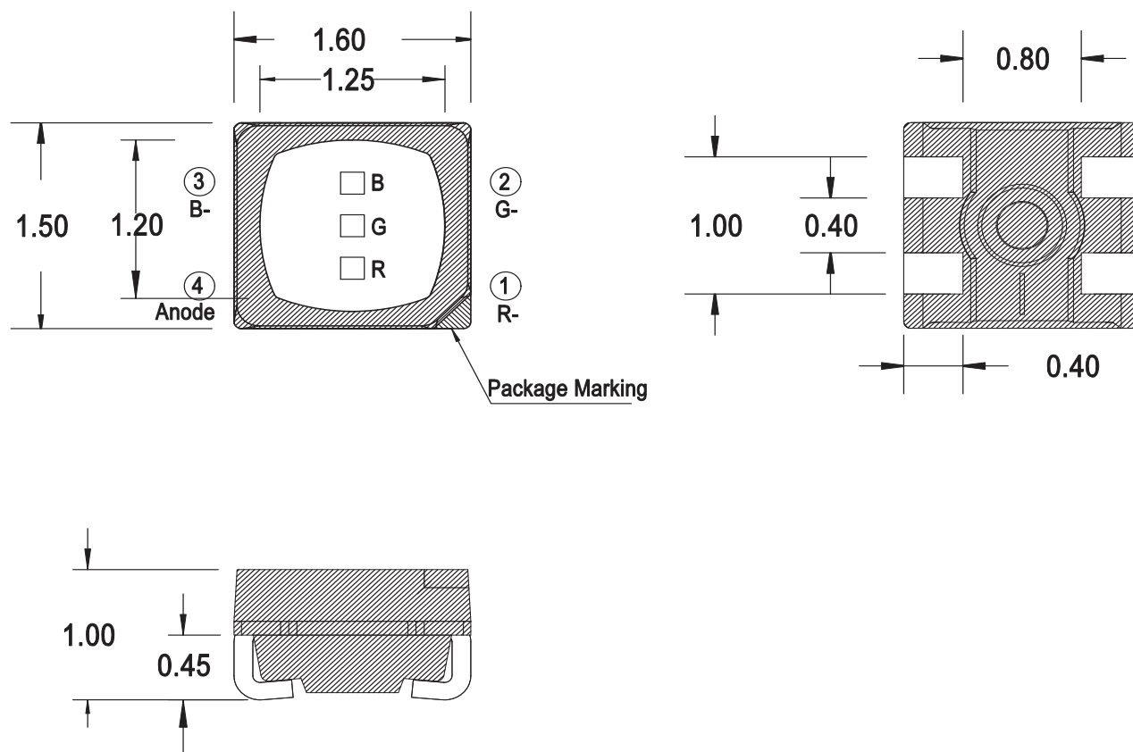
Figure 1: Package Drawing
