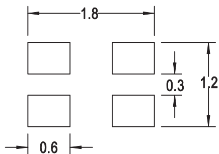
Figure 12: Recommended Soldering Pad Pattern
