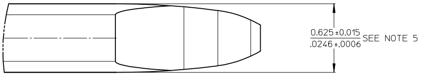
DETAIL "B" SCALE 30:1
