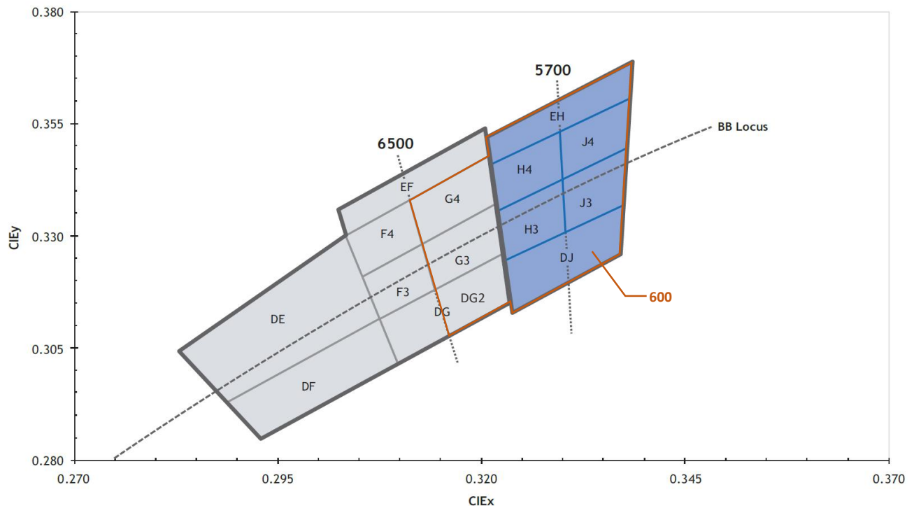
Luminus' Standard Chromaticity Bins: 1931 CIE Curve
