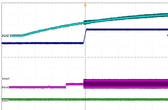
PV IN : 5 V/div, PWM: 5 V/div, V OUT : 200 mV/div, I OUT : 20 A/div
