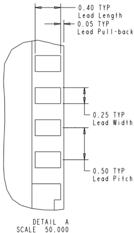
Figure 27: Package Dimensions 3/3
