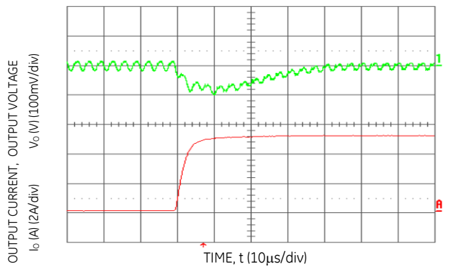
Figure 12. Transient Response to Dynamic Load Change from 50% to 100% of full load (Vo = 3.3 Vdc, Cext = 2x150 µF Polymer Capacitors).
