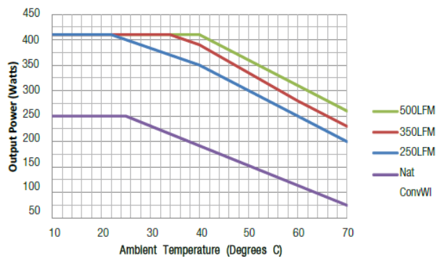
Power Rating at 90Vac
