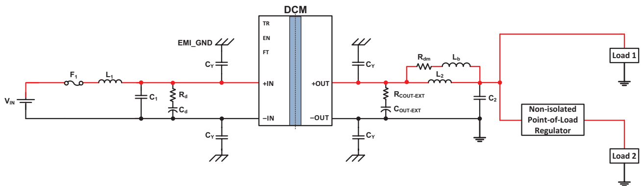
Typical application 2: single DCM3623x50M53C2yzz, to a non-isolated regulator, and direct to load
