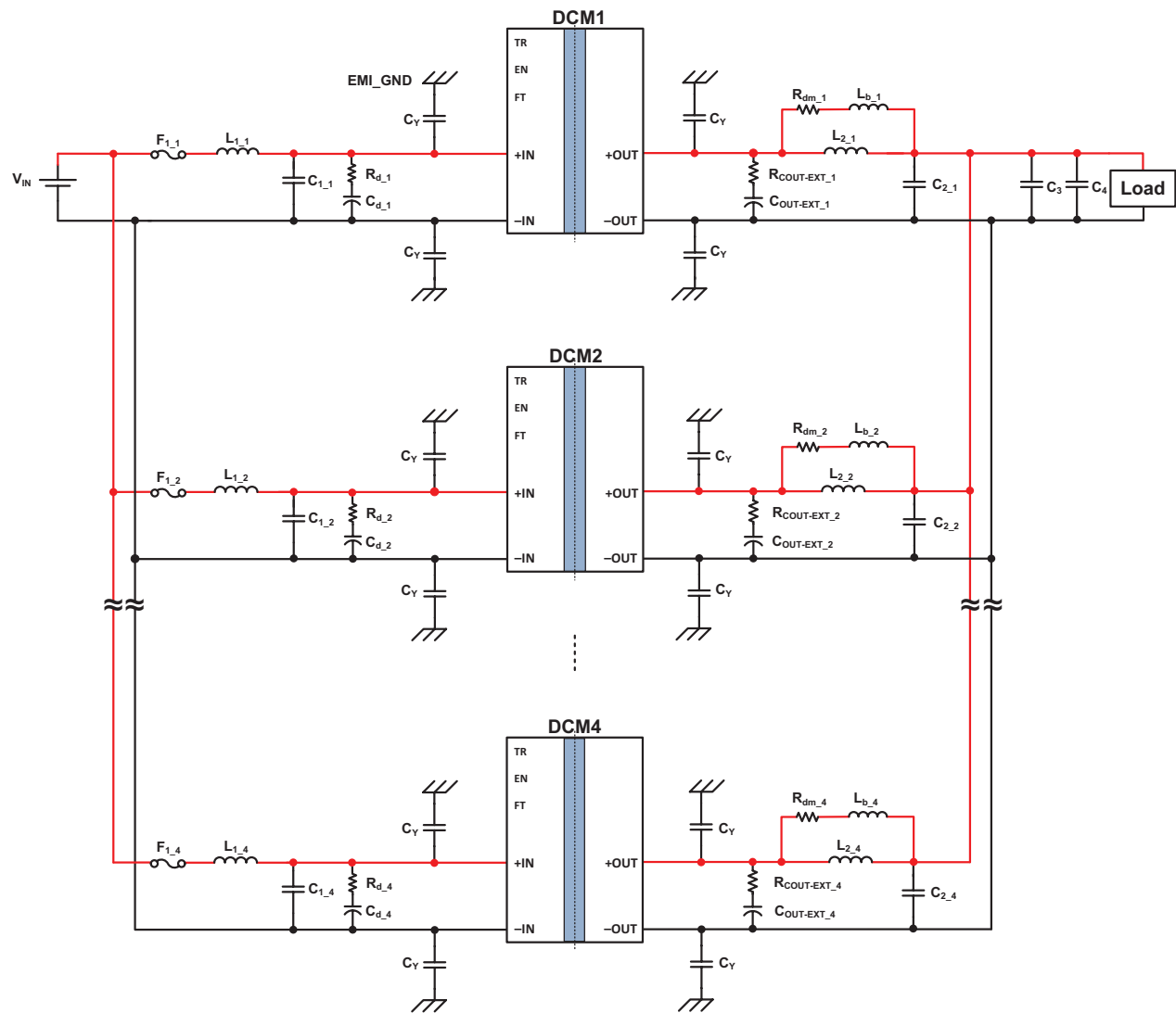
Typical application 1: DCM3623x50M53C2yzz in an array of four units
