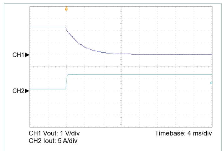
Figure 8 — 10 – 100% load transient response, V_{IN} = 28\text{V} , nominal trim, C_{OUT\_EXT} = 200\mu\text{F}
