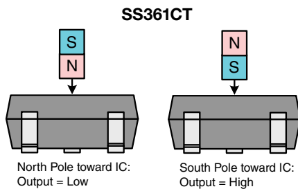
Figure 4. Magnetic Activation
