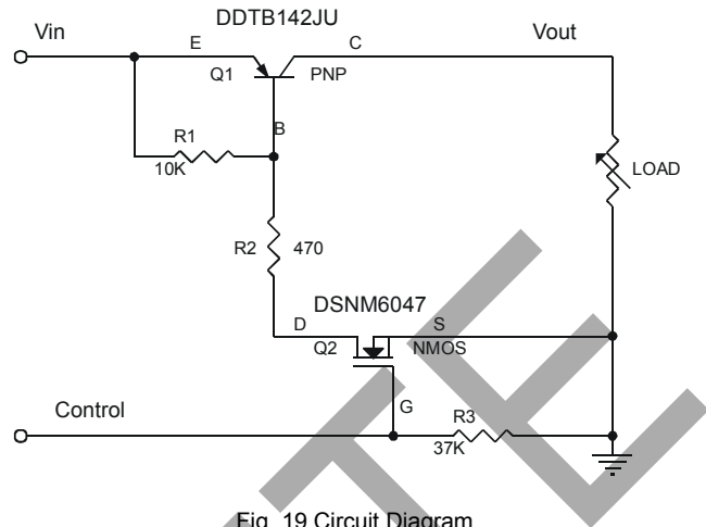
Fig. 19 Circuit Diagram
