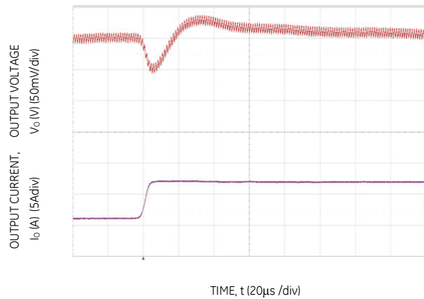
Figure 22. Transient Response to Dynamic Load Change from 50% to 100% at 12Vin, Cout = 2x47uF+1x330uF, CTune=3300pF & RTune=240Ω
