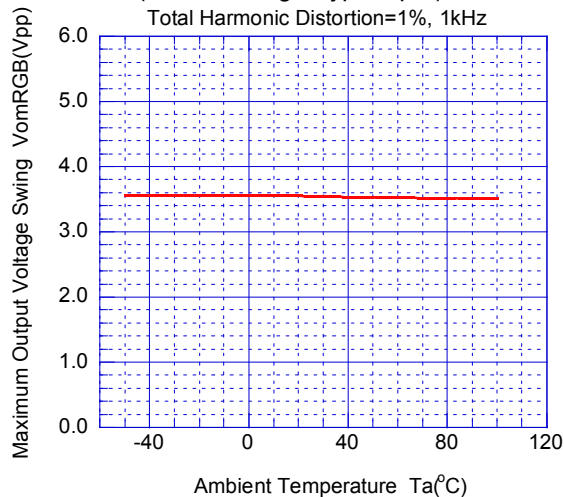
Maximum Output Voltage Swing vs. Temperature (Bias+Through Type Input) Total Harmonic Distortion=1%, 1kHz
