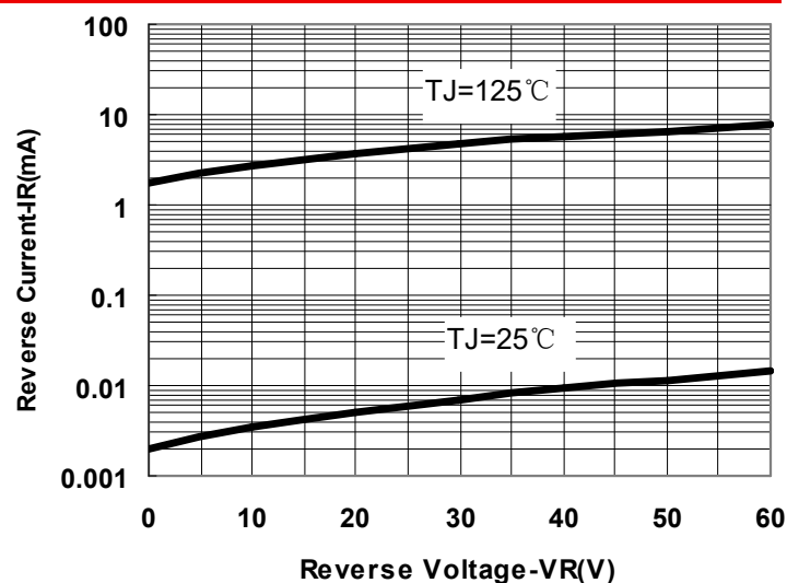
Fig.2-Typical Reverse Characteristics
