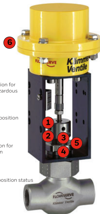
Valve Actuator
