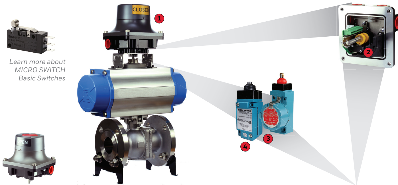
Figure 4. Switches in Valve Actuators and Positioners
