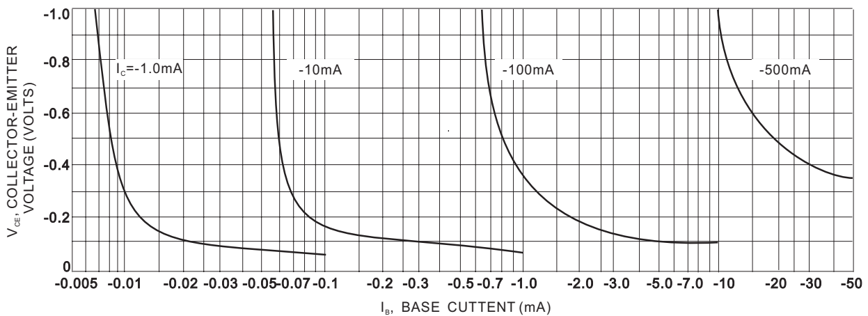
Fig.2-Collector Saturation Region
