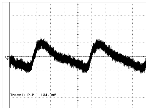
Figure 22 - Ripple, 85 VAC, Full Load. 2 ms, 50 mV / div.
