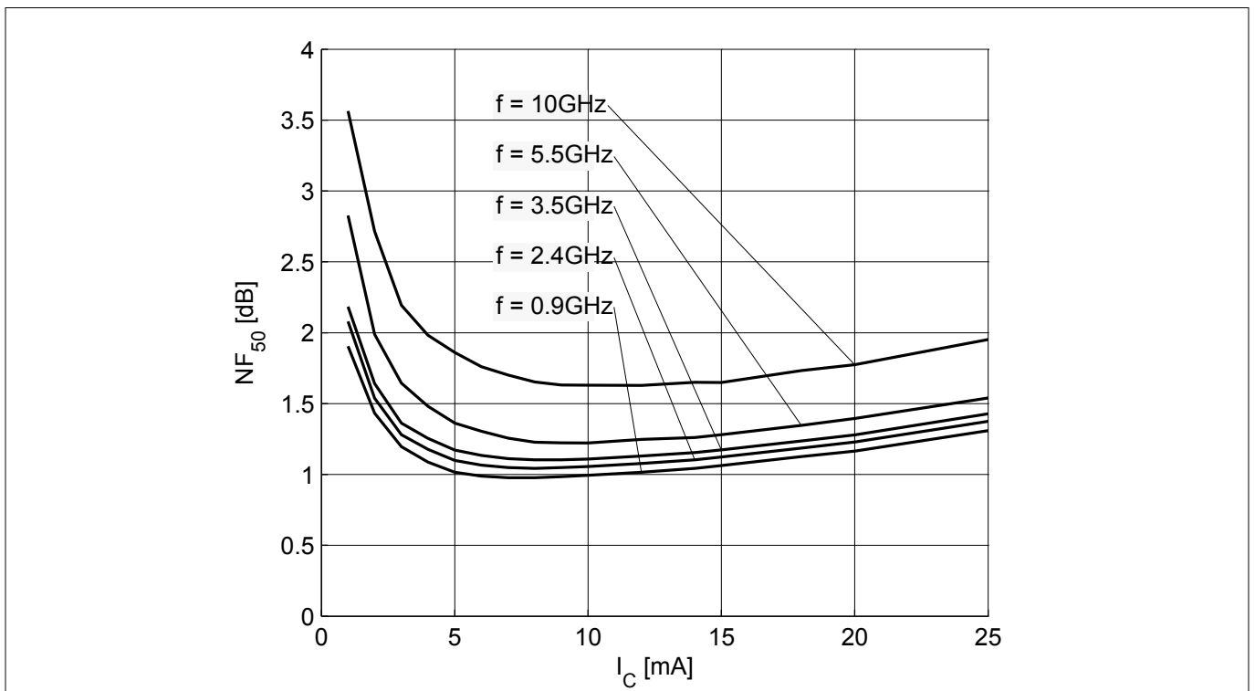
Figure 19 Noise figure NF_{50} = f(I_C) , V_{CE} = 1.8 V , Z_S = 50 \Omega , f = \text{parameter}
