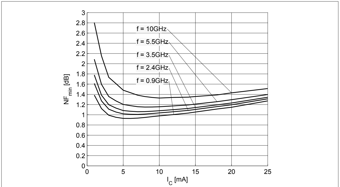
Figure 18 Noise figure NF_{min} = f(I_C) , V_{CE} = 1.8 V , Z_S = Z_{S,opt} , f = \text{parameter}
