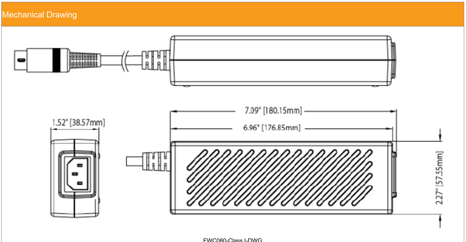
FWC080-Class I-DWG
