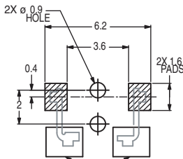
PCB MOUNTING
