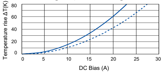
[ ETQP5M2R0YLC ]
