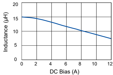
[ ETQP5M150YFK ]
