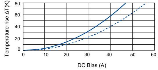
[ ETQP5M1R0YLC ]
