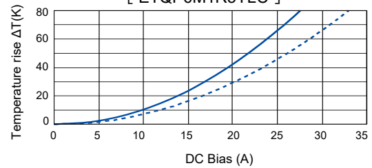
[ ETQP6M1R5YLC ]
