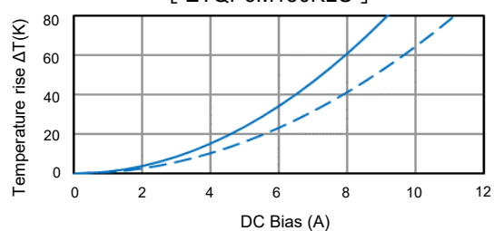
[ ETQP6M150KLC ]
