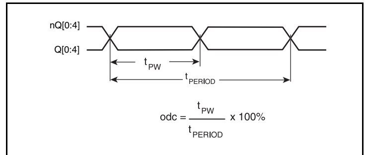
Output Duty Cycle/Pulse Width/Period
