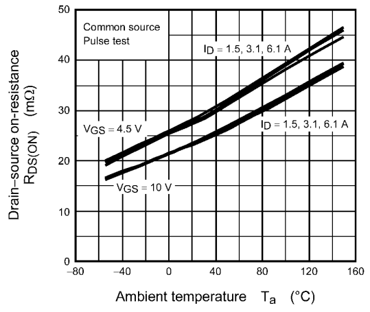
Fig. 8.2.6 R_{DS(ON)} - T_a
