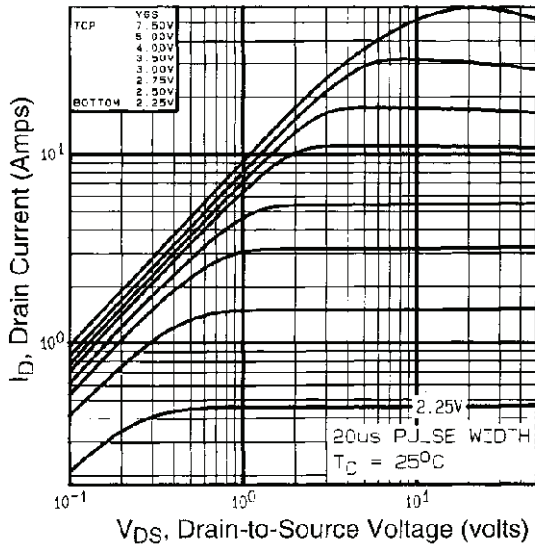
Fig. 1 - Typical Output Characteristics, T_C = 25^\circ\text{C}
