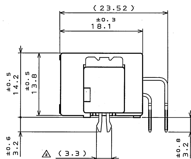
△2 P.C.B. HOLE PATTERNS(REF.) (NOTE6&TABLE1)
