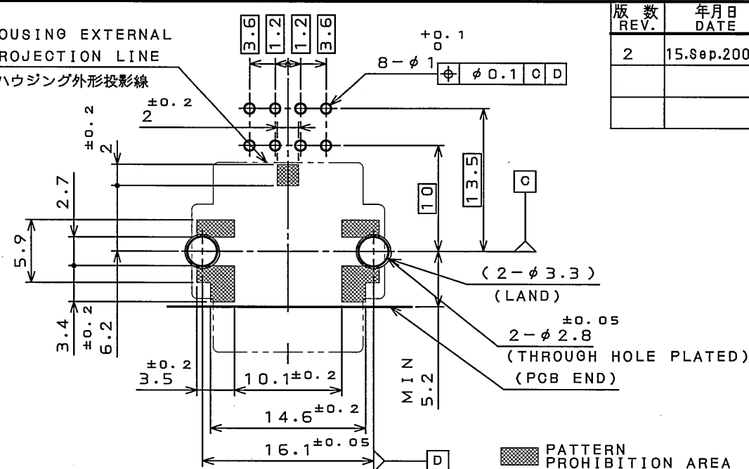
△2 P.C.B. HOLE PATTERNS(REF.) (NOTE6&TABLE1)
