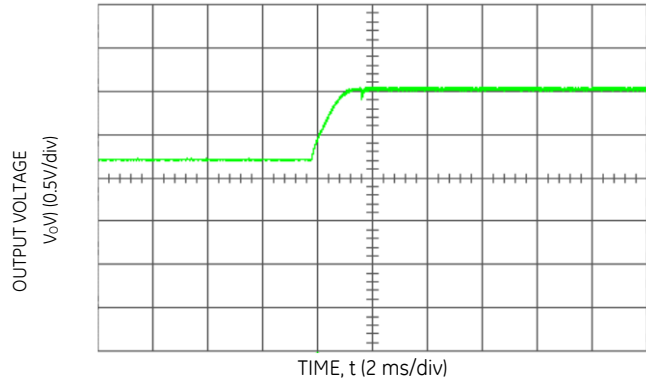
Figure 17 Typical Start-Up with Prebias ( V_{in} = 12\text{ Vdc} , V_o = 5.0\text{ Vdc} , I_o = 1\text{ A} , V_{bias} = 3.3\text{ Vdc} ).
