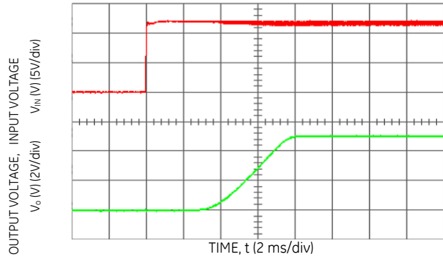
Figure 16. Typical Start-Up with application of V_{in} with low-ESR polymer capacitors at the output ( 7 \times 150\ \mu\text{F} ) ( V_{in} = 12\text{ Vdc} , V_o = 5.0\text{ Vdc} , I_o = 16\text{ A} , C_o = 1050\ \mu\text{F} ).
