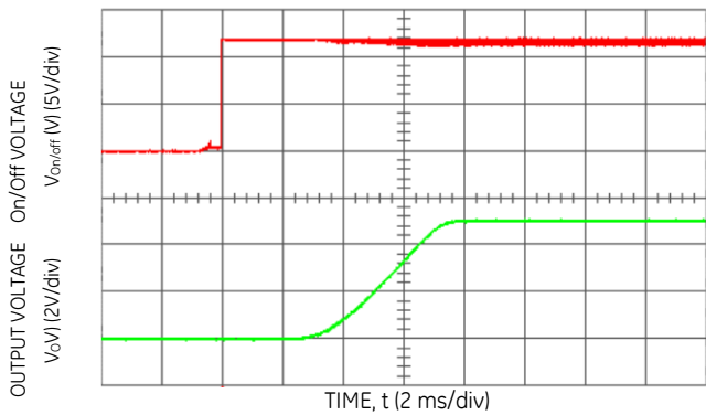
Figure 15. Typical Start-Up Using Remote On/Off with Low-ESR external capacitors ( 7 \times 150\ \mu\text{F} Polymer) ( V_{in} = 12\text{ Vdc} , V_o = 5.0\text{ Vdc} , I_o = 16\text{ A} , C_o = 1050\ \mu\text{F} ).
