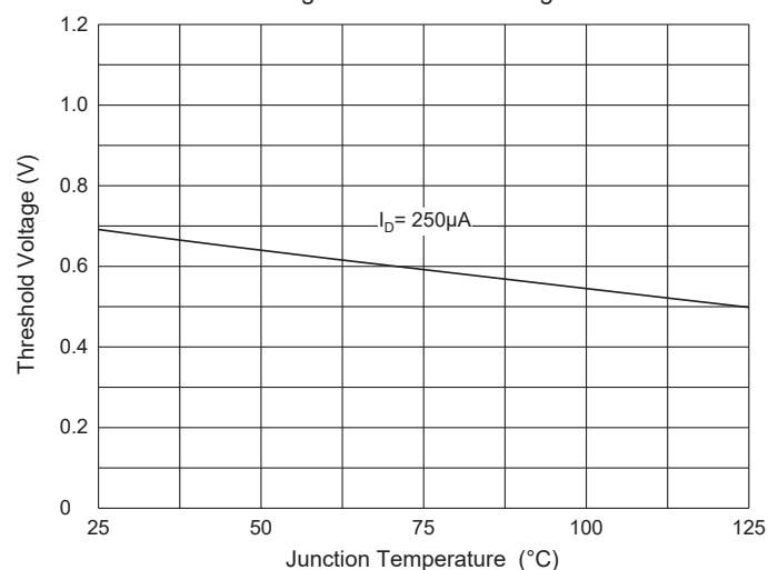
Fig. 4 - Threshold Voltage
