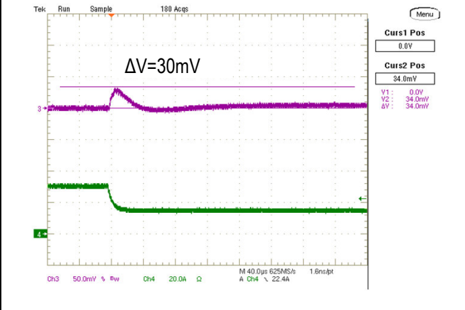
Step Load Transient Response (Vin=12.0V, Vout=0.7V, Cload=760uF, Iout=30 to 15A, 1.0A/us) Trace 3=Vout, 50mV/div, Trace 4=Iout, 20A/div.
