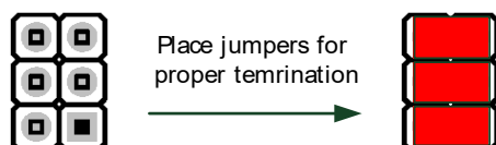
Figure 3.3 Encoder input termination
