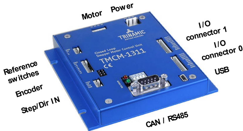
Figure 3.2 TMC1311 connectors
