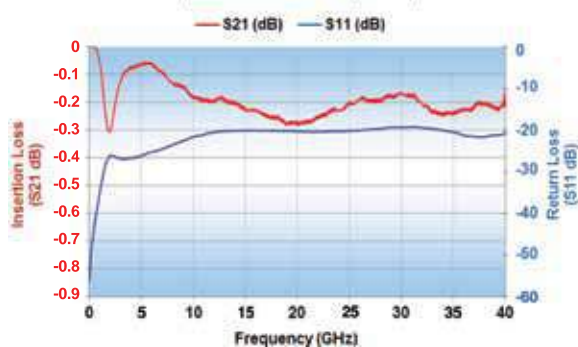
P42BN300MA3182 Opti-Cap Typical Performance (Reference 50 Ohm System)
