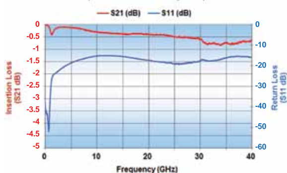
P62BN300MA2636 Opti-Cap Typical Performance (Reference 50 Ohm System)
