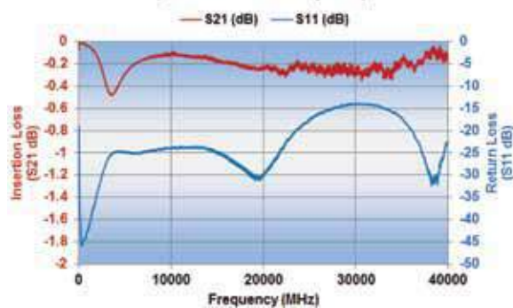
P21BN300MA4678 Opti-Cap Typical Performance (Reference 50 Ohm System)
