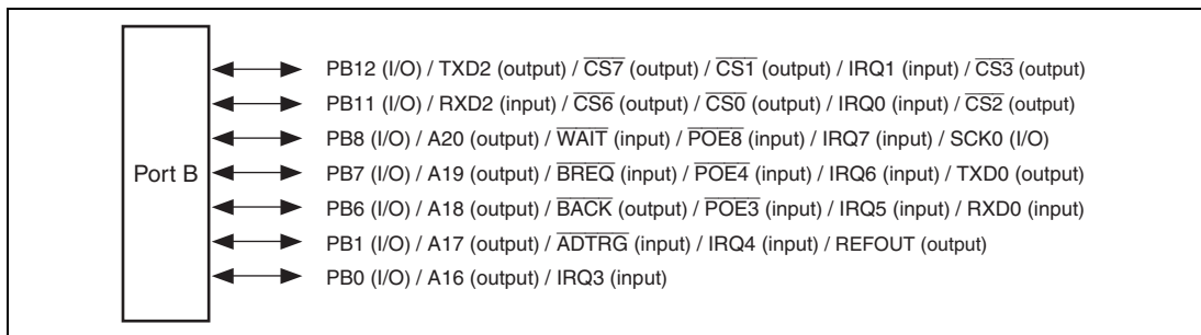
Figure 24.4 Port B (SH7243)
