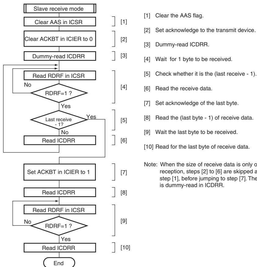
Figure 19.22 Sample Flowchart for Slave Receive Mode
