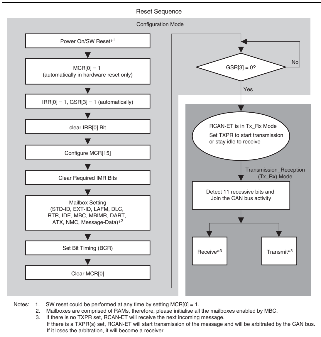
Figure 22.8 Reset Sequence
