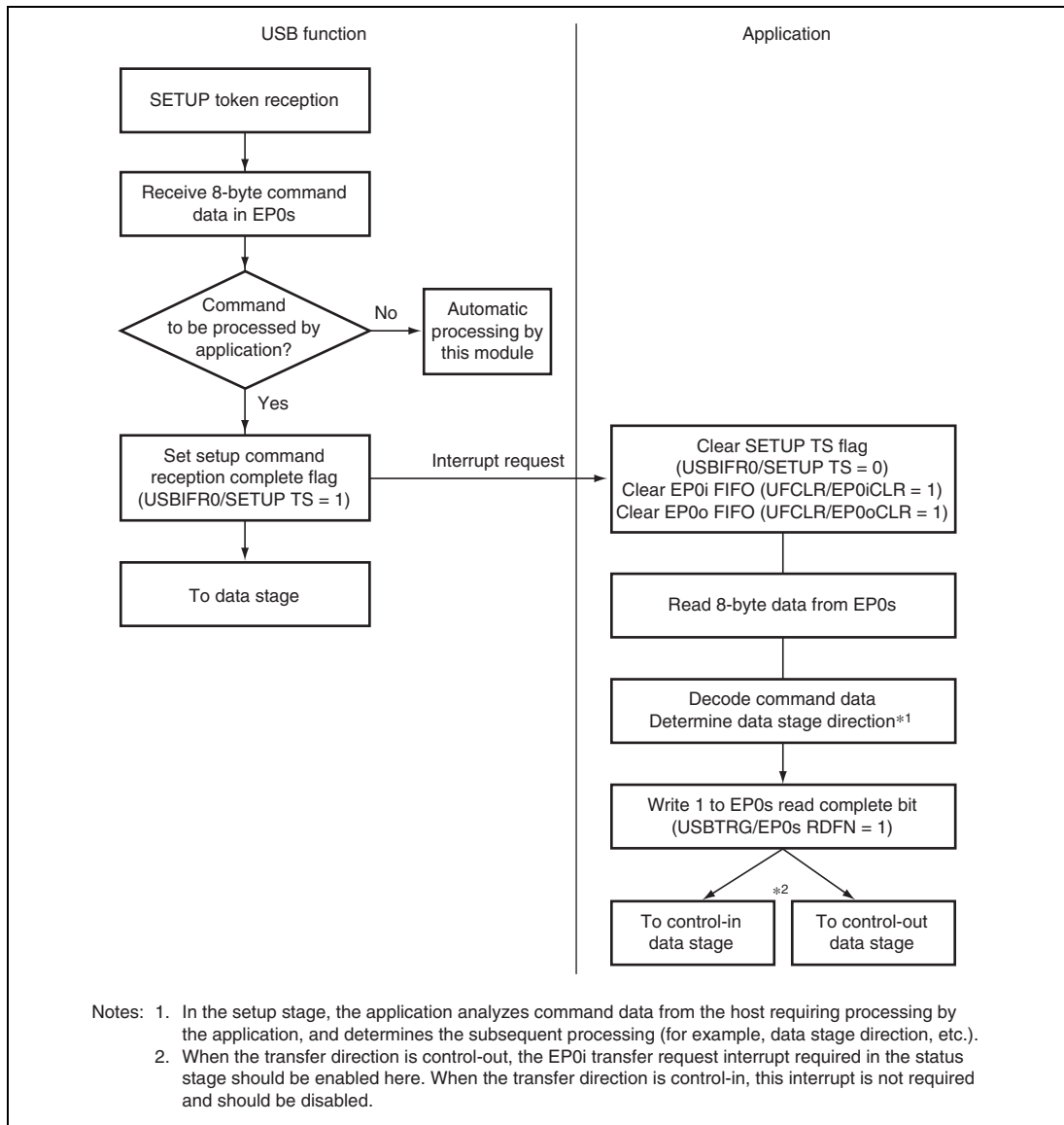
Figure 25.6 Setup Stage Operation
