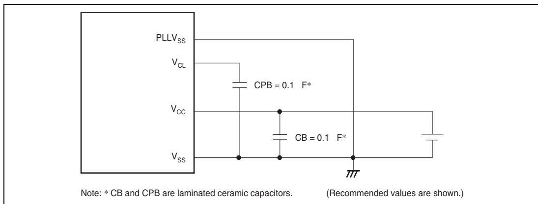
Figure 4.10 Recommended External Circuitry around PLL
