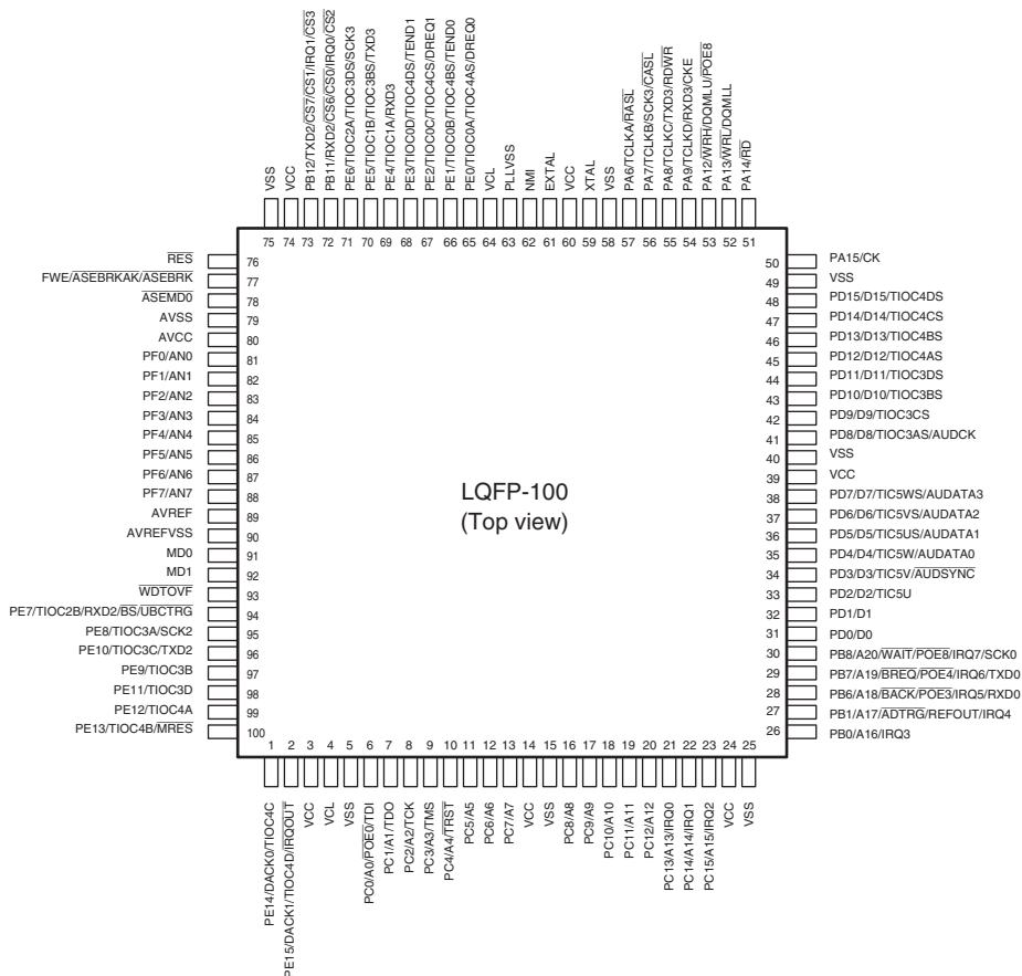
Figure 1.5 SH7243 Pin Assignment
