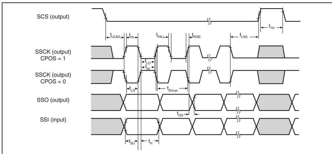
Figure 31.50 SSU Timing (Master, CPHS = 0)
