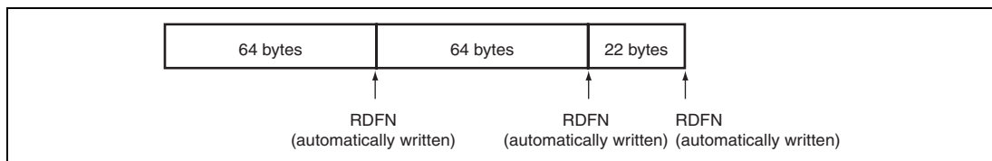
Figure 25.16 EP1 RDFN Operation
