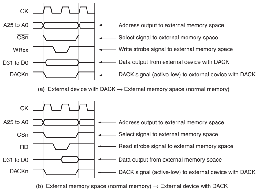
Figure 10.8 Example of DMA Transfer Timing in Single Address Mode
