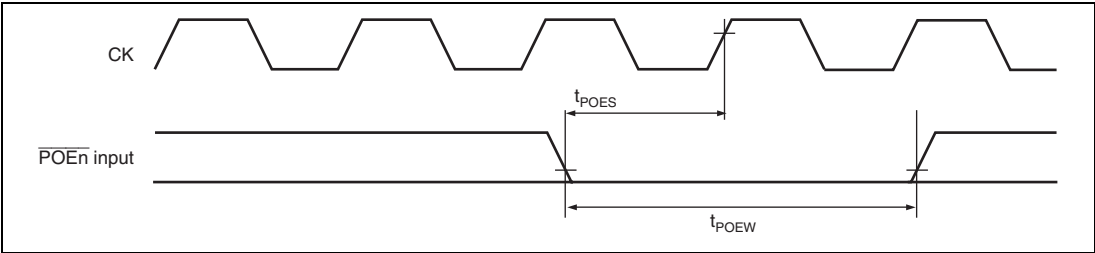
Figure 31.43 POE2 Input/Output Timing
