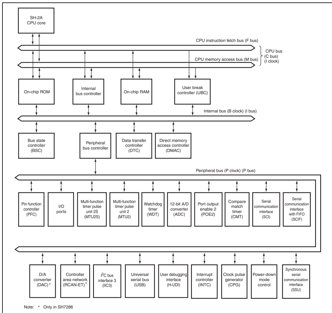
Figure 1.2 Block Diagram (SH7285, SH7286)
