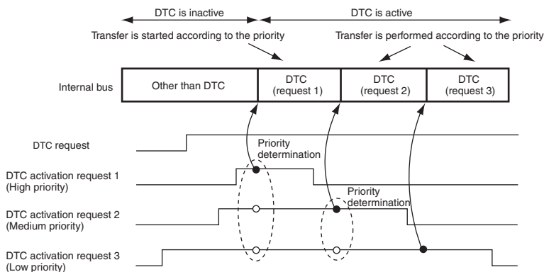
Figure 8.17 Example of DTC Activation According to Priority
