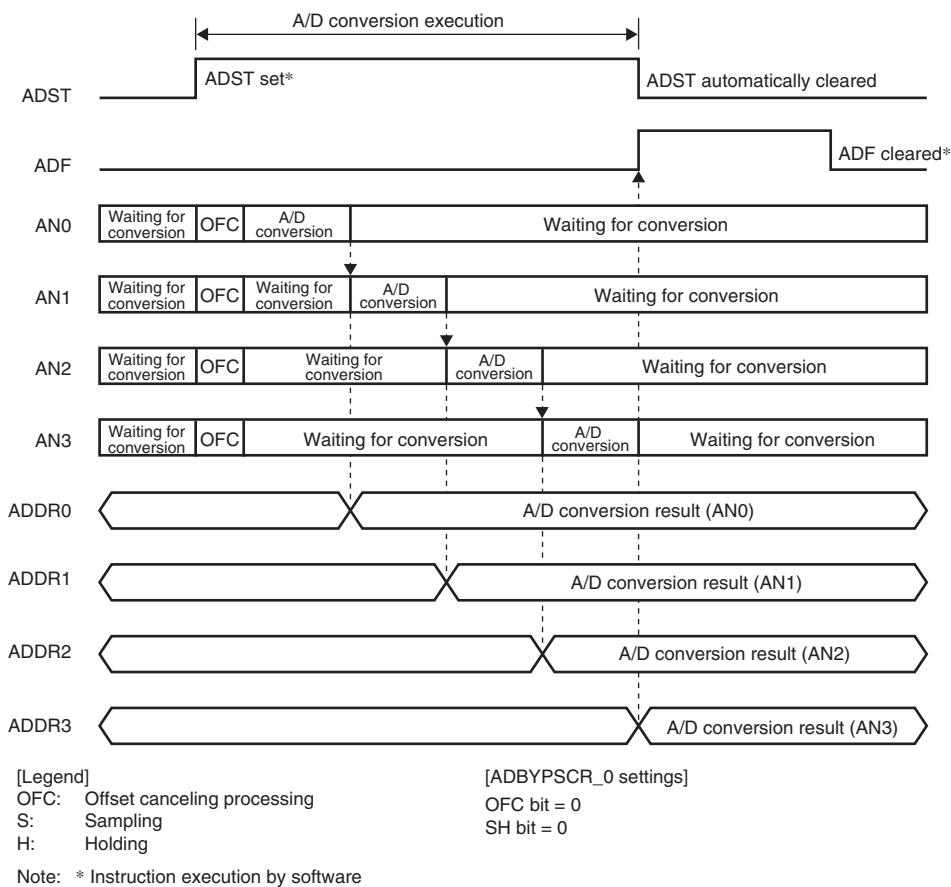
Figure 20.3 Example 2 of A/D_0 Converter Operation (Single-Cycle Scan Mode, Sample-and-Hold Circuit Disabled, and Offset Canceling Circuit Enabled)
