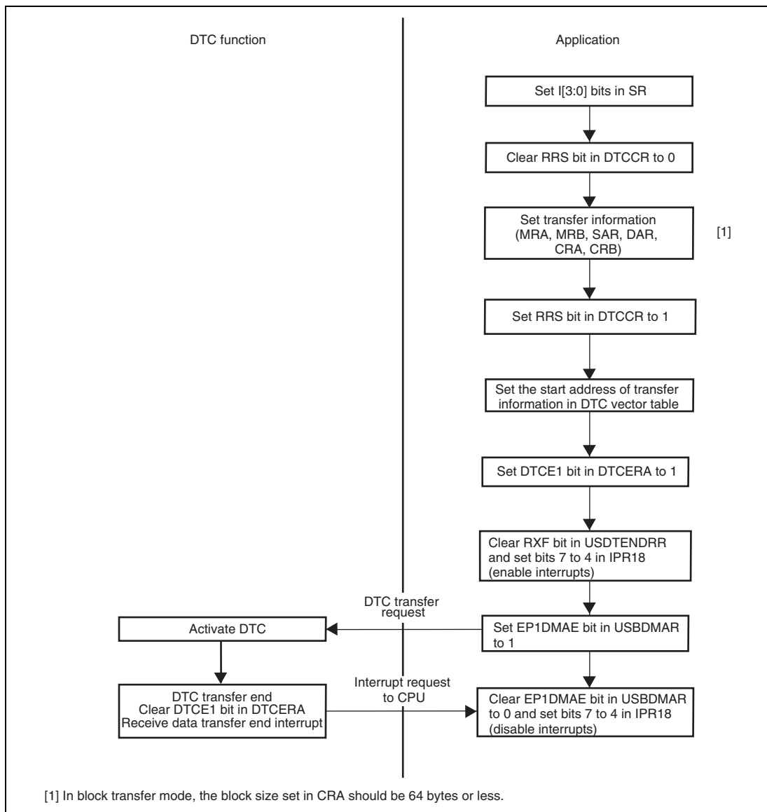
Figure 25.23 Example of DTC Transfer for Bulk-OUT Transfer (EP1) (When Receive Data Size is Determined Before Receiving Out Token)
