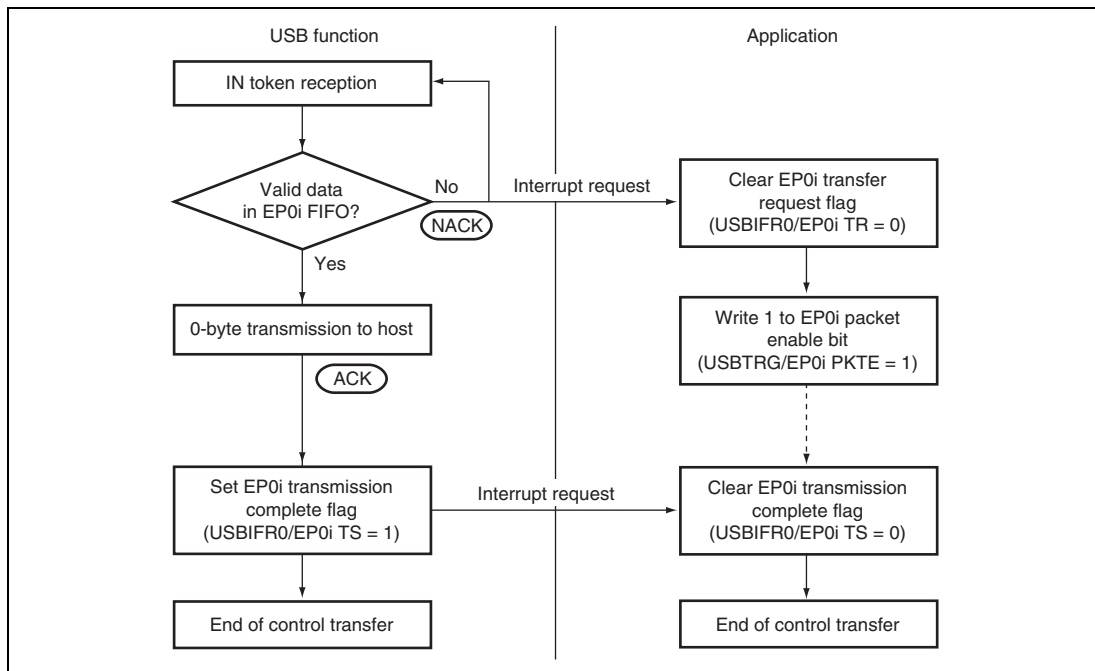
Figure 25.10 Status Stage (Control-OUT) Operation
