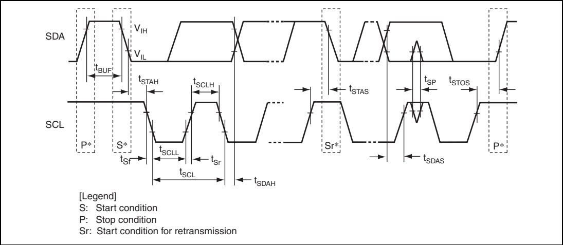
Figure 31.54 I²C Bus Interface 3 Input/Output Timing
