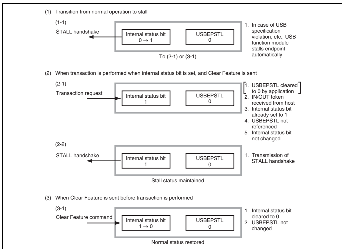
Figure 25.15 Automatic Stall by USB Function Module
