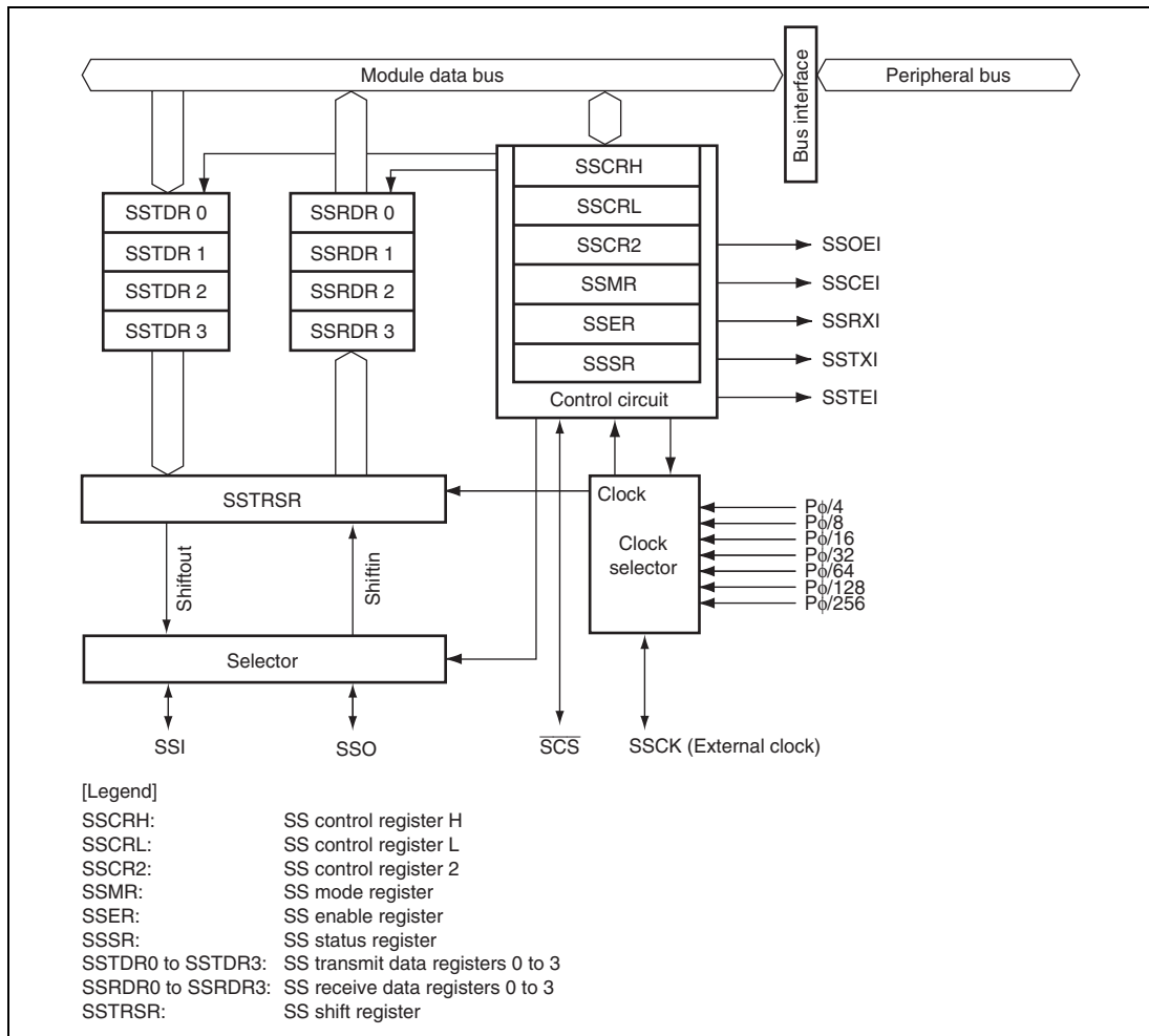
Figure 18.1 Block Diagram of SSU
