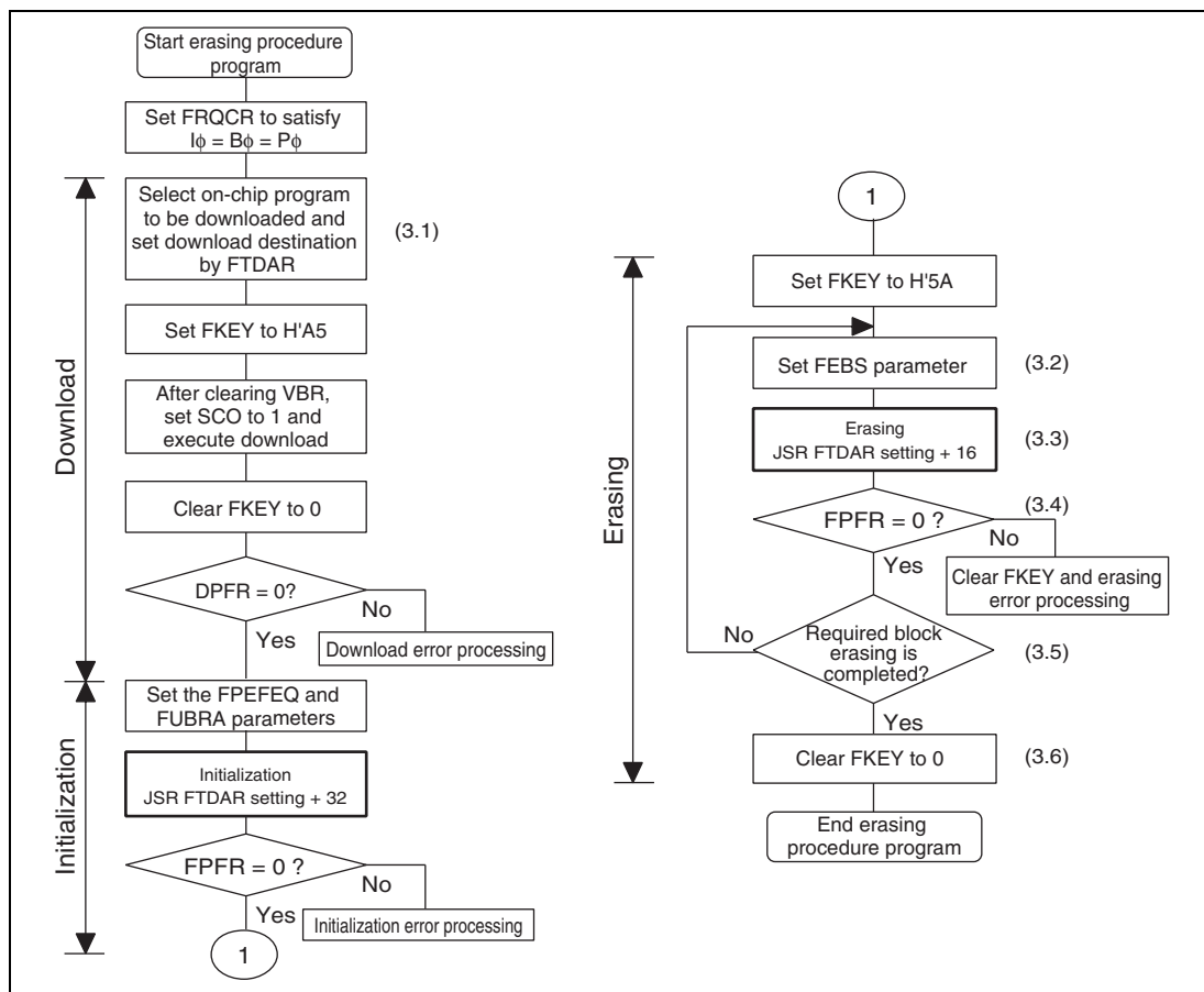
Figure 26.14 Erasing Procedure
