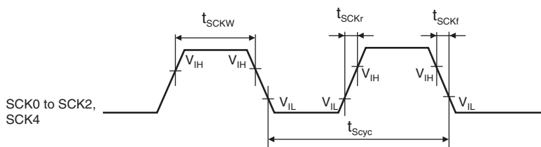
Figure 31.45 Input Clock Timing
