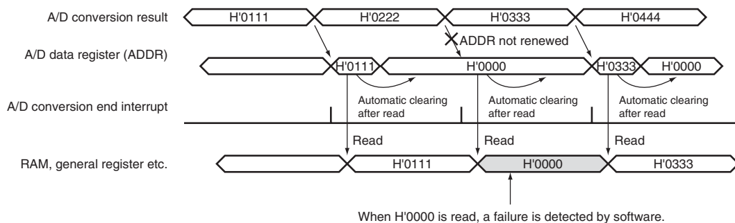
Figure 20.12 Example of When ADDR Auto-clear Function is Disabled (Normal Condition)/Enabled
