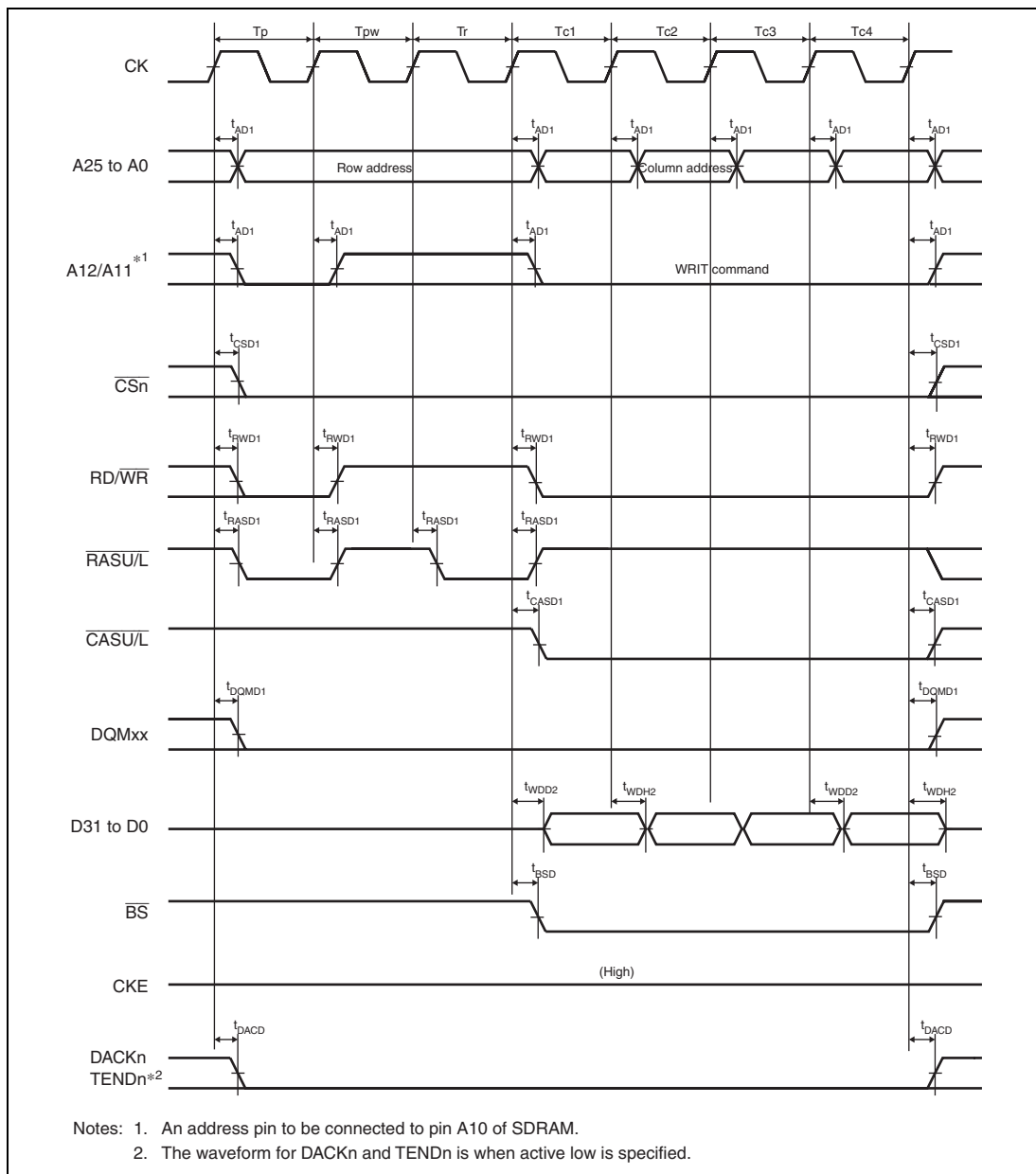
Figure 31.31 Synchronous DRAM Burst Write Bus Cycle (Four Write Cycles) (Bank Active Mode: PRE + ACT + WRITE Commands, Different Row Addresses, WTRCD = 0 Cycle, TRWL = 0 Cycle)
