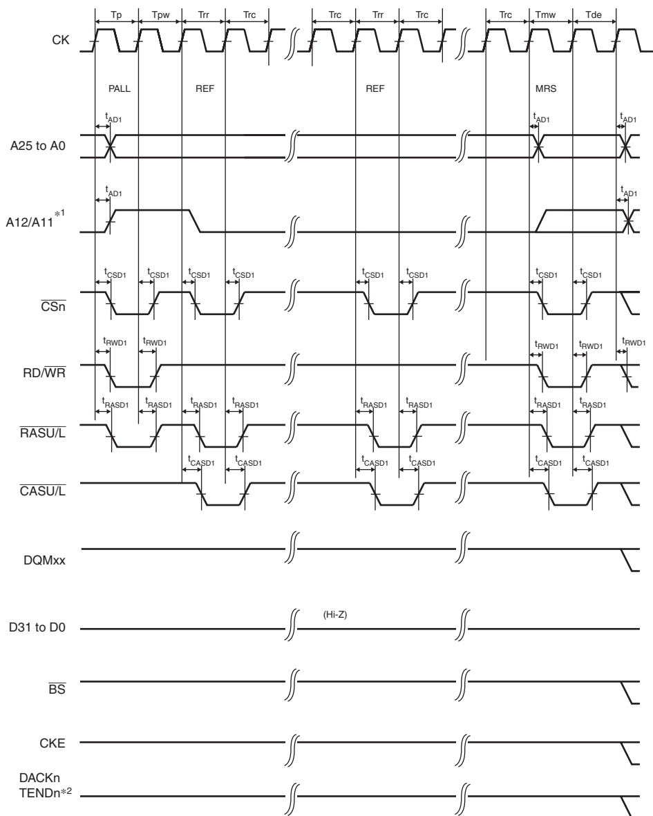
Figure 31.34 Synchronous DRAM Mode Register Write Timing (WTRP = 1 Cycle)
