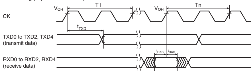
Figure 31.46 SCI Input/Output Timing
