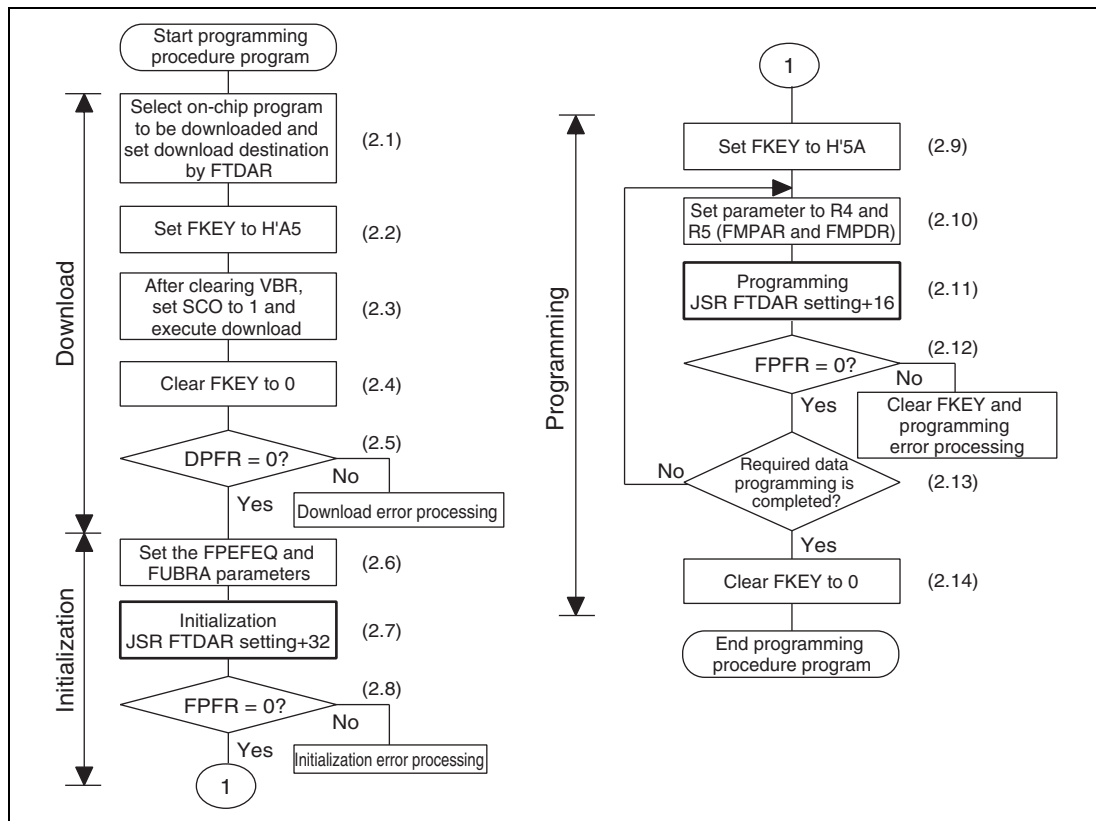
Figure 26.13 Programming Procedure
