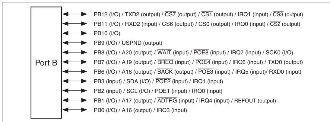
Figure 24.5 Port B (SH7285)
