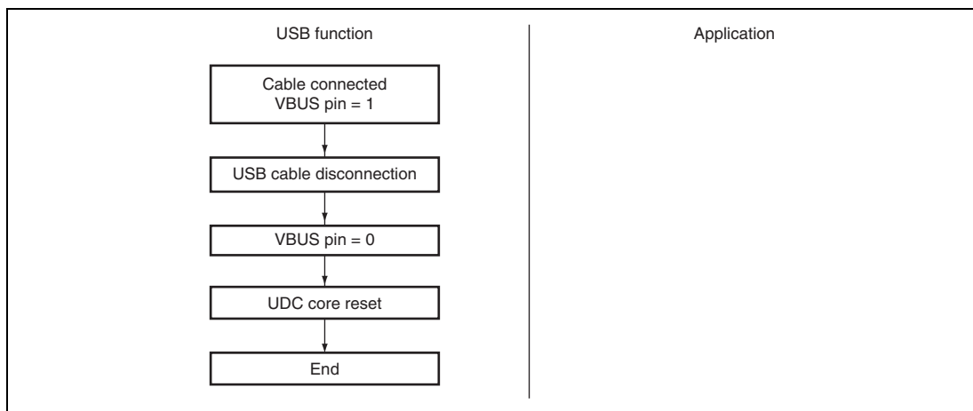
Figure 25.4 Cable Disconnection Operation
