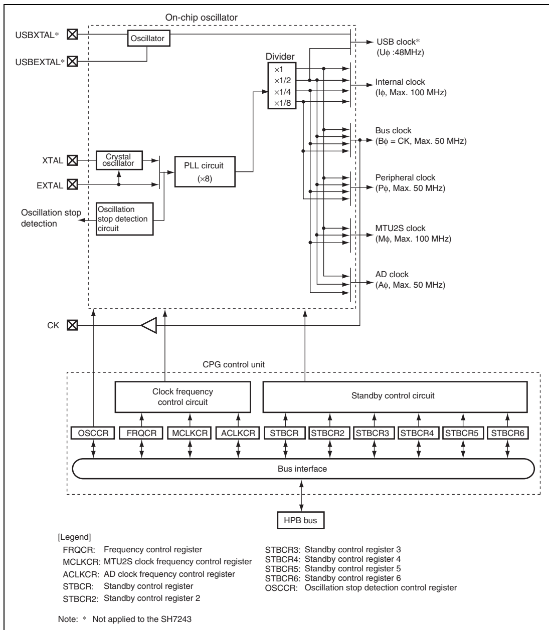
Figure 4.1 Block Diagram of Clock Pulse Generator
