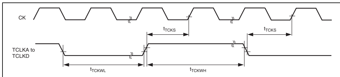
Figure 31.41 MTU2 Clock Input Timing
