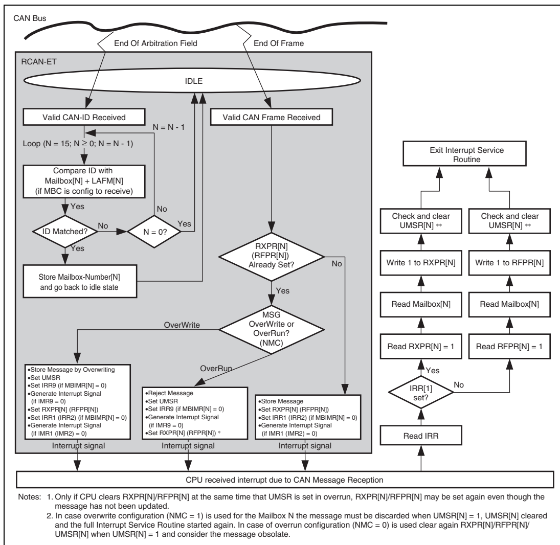
Figure 22.12 Message Receive Sequence
