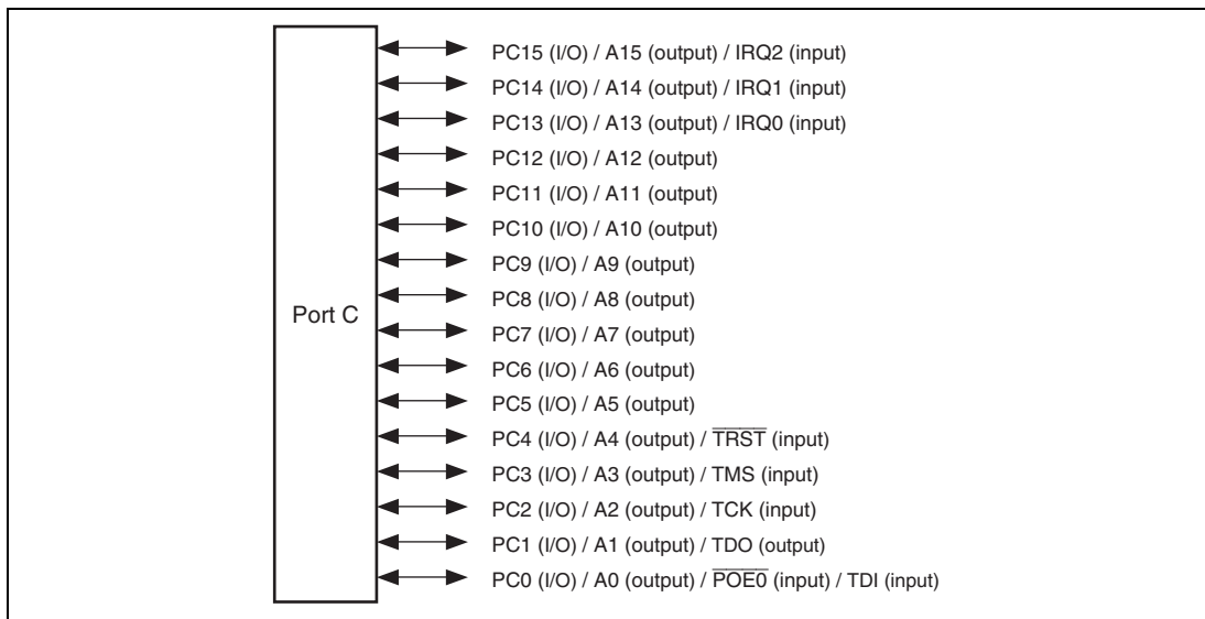
Figure 24.7 Port C (SH7243)
