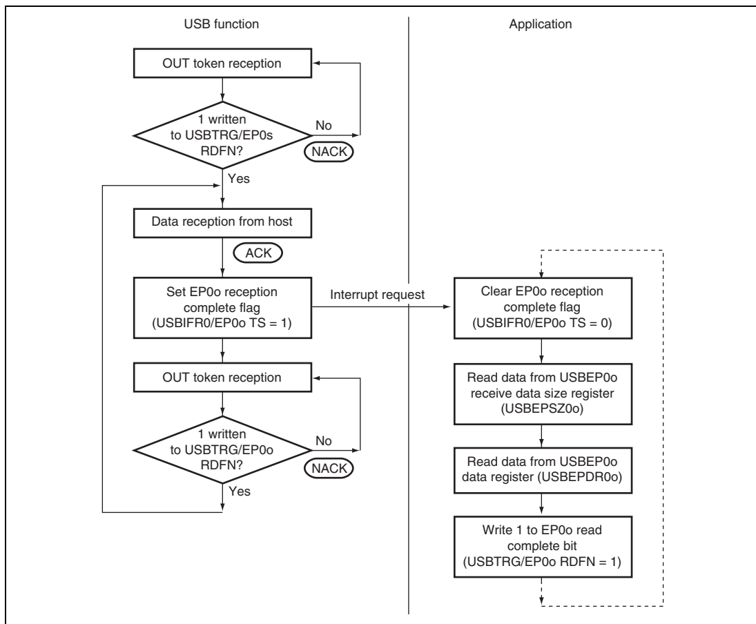
Figure 25.8 Data Stage (Control-OUT) Operation
