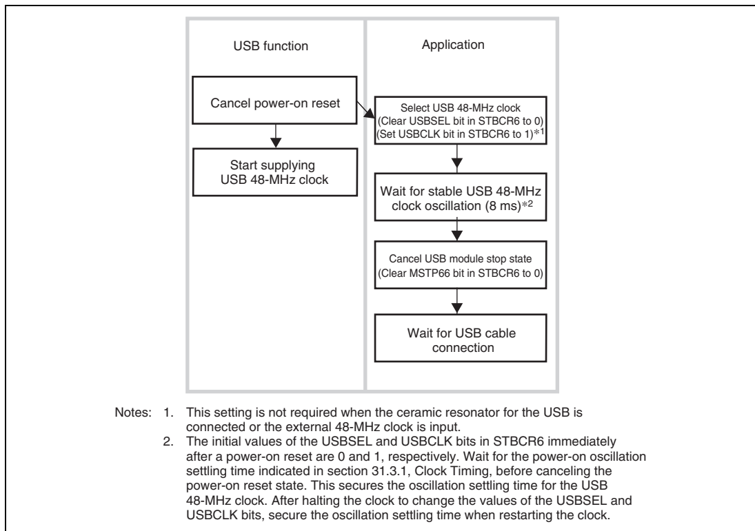
Figure 25.2 Initial Setting Operation
