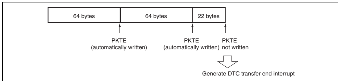
Figure 25.25 EP2 PKTE Operation
