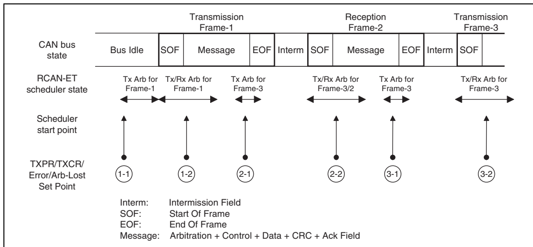
Figure 22.11 Internal Arbitration for Transmission
