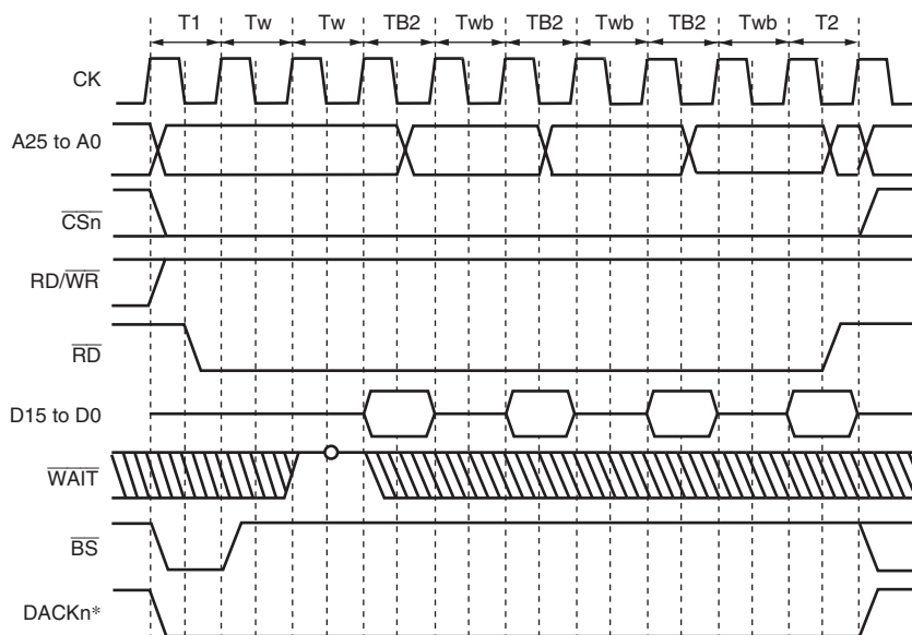
Figure 9.35 Burst ROM Access Timing (Clock Asynchronous)
