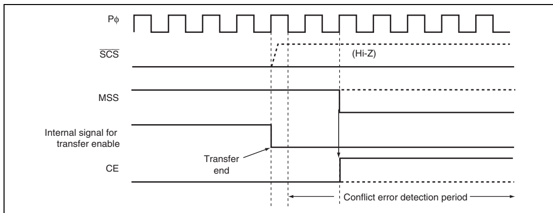
Figure 18.11 Conflict Error Detection Timing (After Transfer End)
