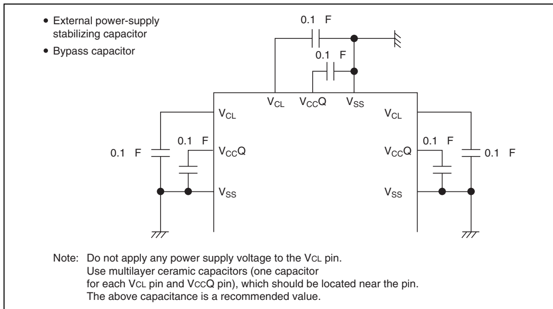
Figure 31.62 Connection of Capacitors
