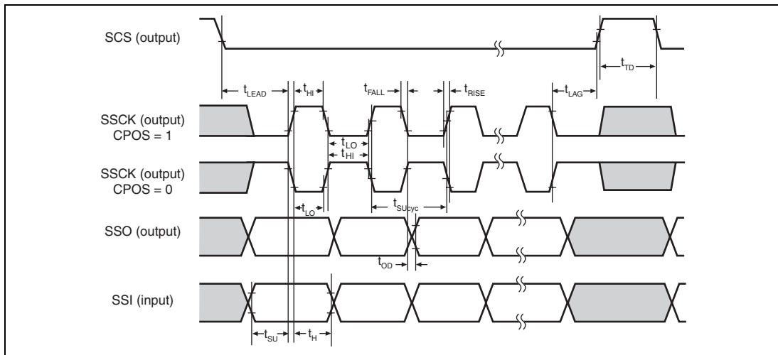
Figure 31.49 SSU Timing (Master, CPHS = 1)
