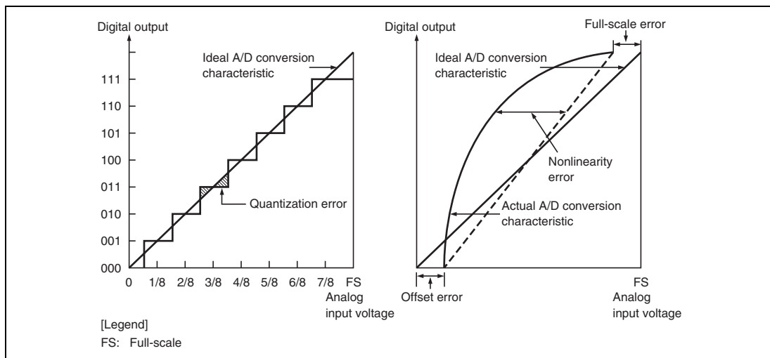
Figure 20.13 Definitions of A/D Conversion Accuracy
