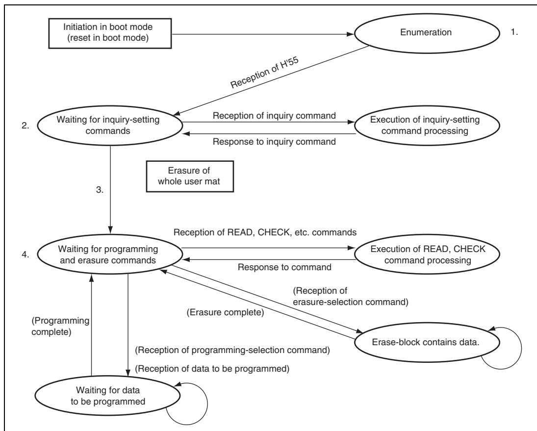
Figure 26.10 USB Boot Mode
