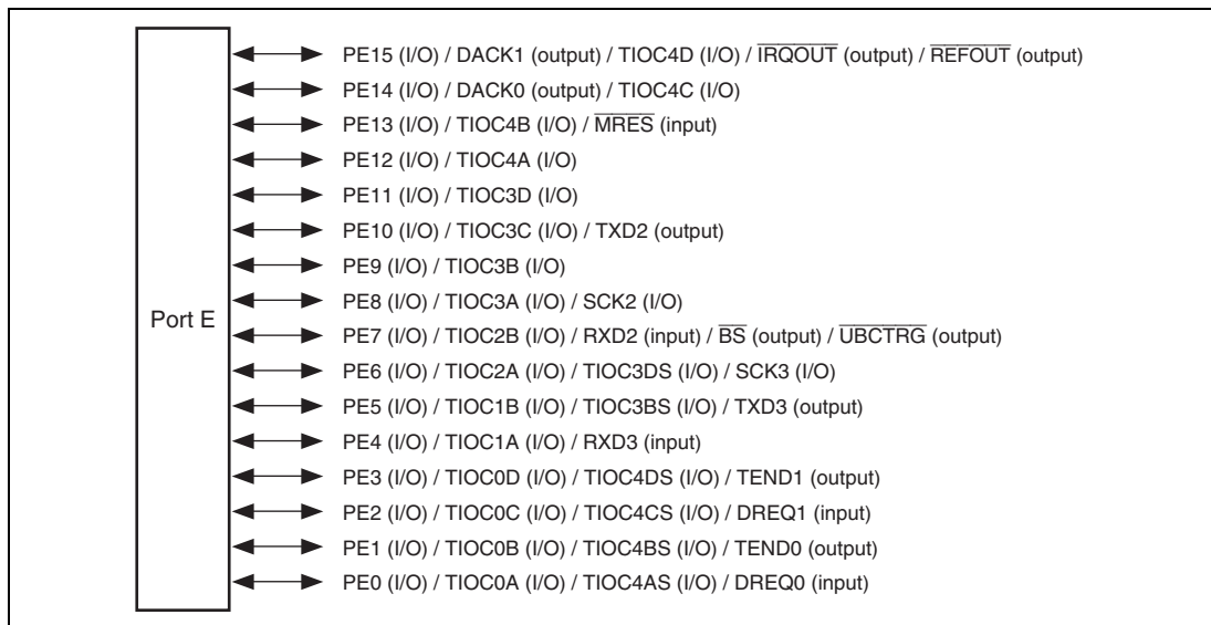
Figure 24.12 Port E (SH7243)
