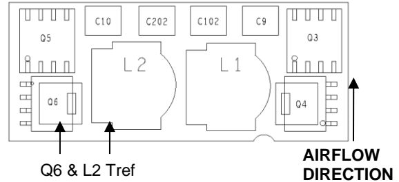
Figure 36. Preferred airflow direction and location of hot-spot of the module ( T_{ref} ).
