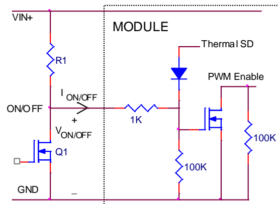
Figure 30. Remote On/Off Implementation using ON/OFF .
