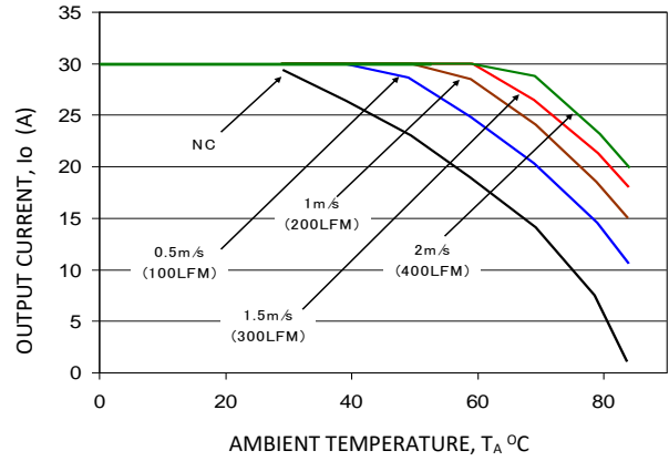
Figure 22. Output Current Derating versus Ambient Temperature and Airflow at 12V in.
