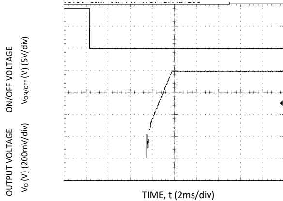
Figure 3. Typical Start-up Using On/Off Voltage ( I_o = I_{o,max} ).
