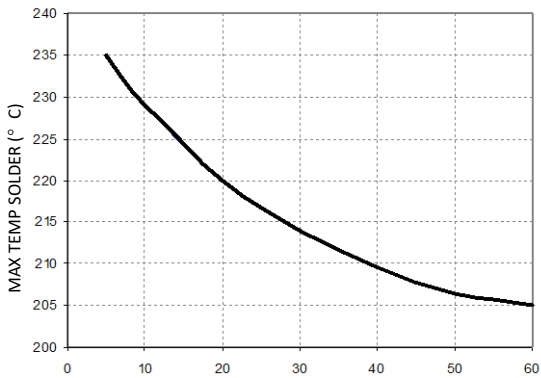
Figure 39. Time Limit Curve Above 205°C Reflow for Tin Lead (Sn/Pb) process.
