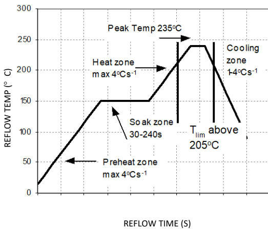
Figure 38. Reflow Profile for Tin/Lead (Sn/Pb) process.
