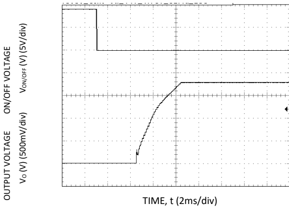
Figure 15. Typical Start-up Using On/Off Voltage ( I_o = I_{o,max} ).
