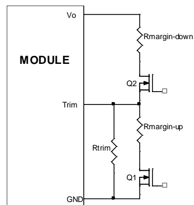
Figure 32. Circuit Configuration for margining Output voltage.
