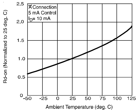
Figure 4. Typical Normalized On-Resistance
