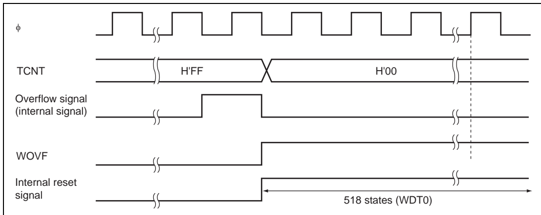
Figure 10.3 Timing of WOVM Setting
