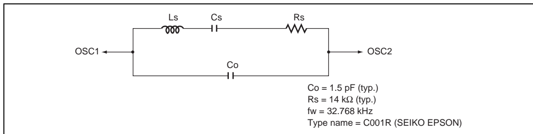
Figure 19.7 Equivalence Circuit for 32.768-kHz Oscillator
