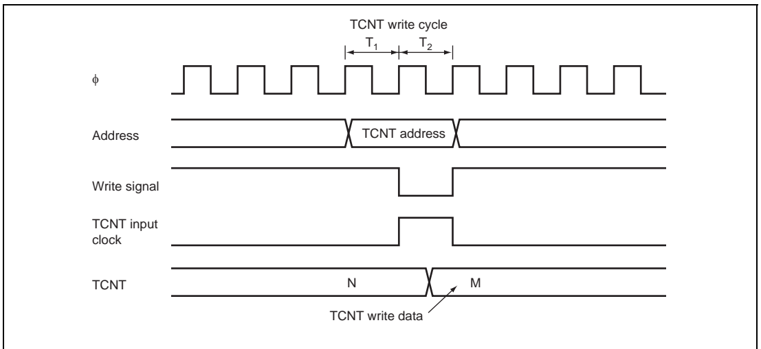
Figure 9.46 Contention between TCNT Write and Increment Operations
