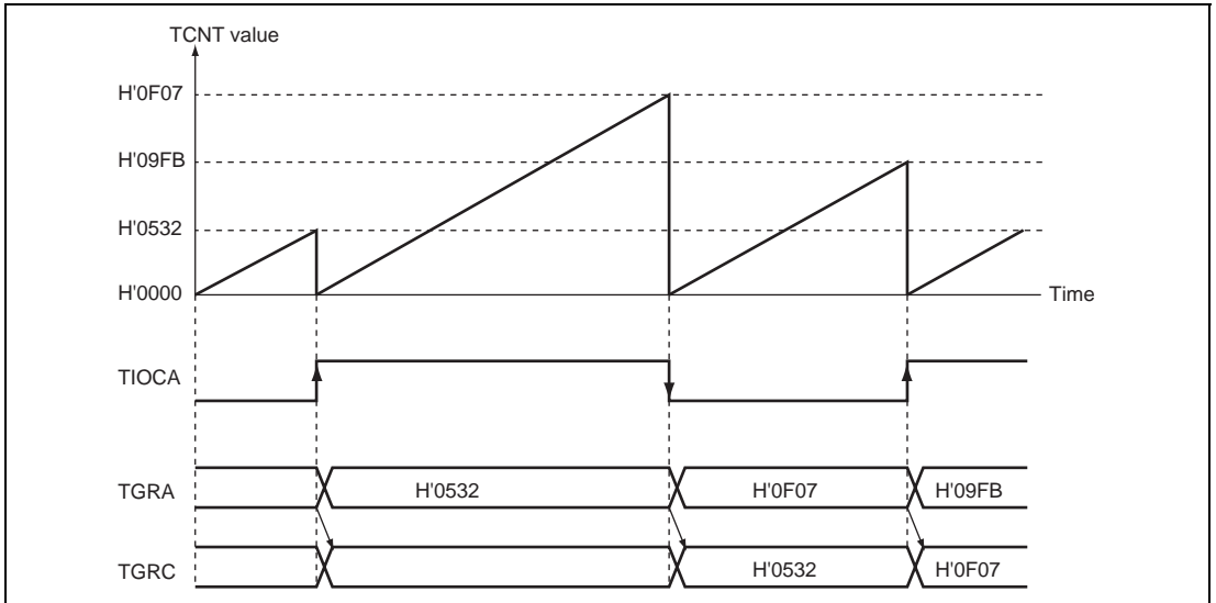
Figure 9.20 Example of Buffer Operation (2)
