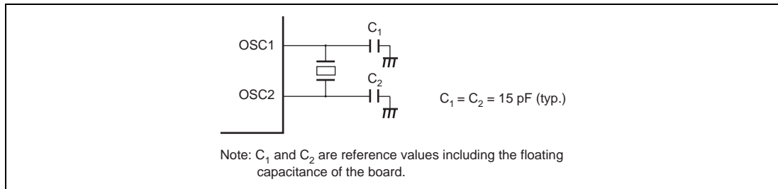
Figure 19.6 Example Connection of 32.768-kHz Quartz Oscillator
