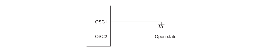
Figure 19.8 Pin Handling when Subclock Not Required
